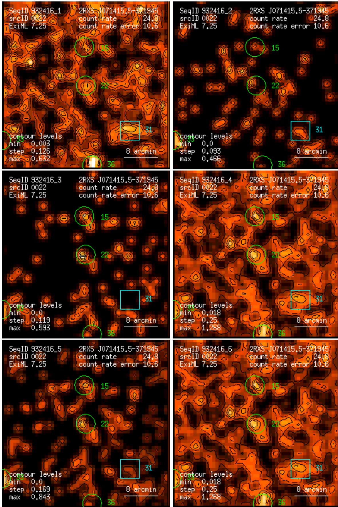
Figure 22: RASS 932416: detection 0022: band rate images, Gaussian filter: (1) PSPC channels 11 – 41, (2) 52 – 90, (3) 91 – 201, (4) 11 – 235, (5) 52 – 201, (6) 11 – 201. Broad band rates in counts/ks. Band rate contour levels in counts/ks/arcmin 2 .
