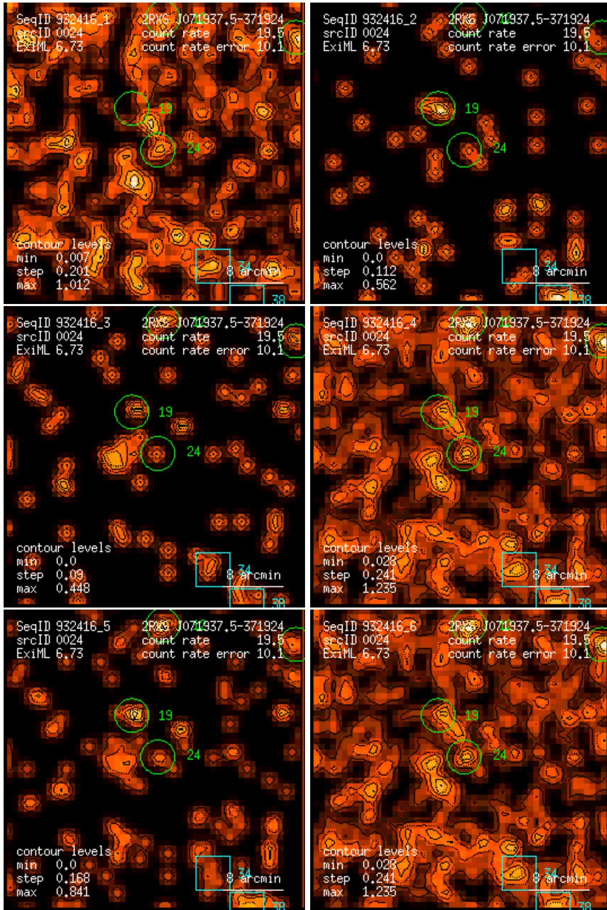
Figure 24: RASS 932416: detection 0024: band rate images, Gaussian filter: (1) PSPC channels 11 – 41, (2) 52 – 90, (3) 91 – 201, (4) 11 – 235, (5) 52 – 201, (6) 11 – 201. Broad band rates in counts/ks. Band rate contour levels in counts/ks/arcmin 2 .
