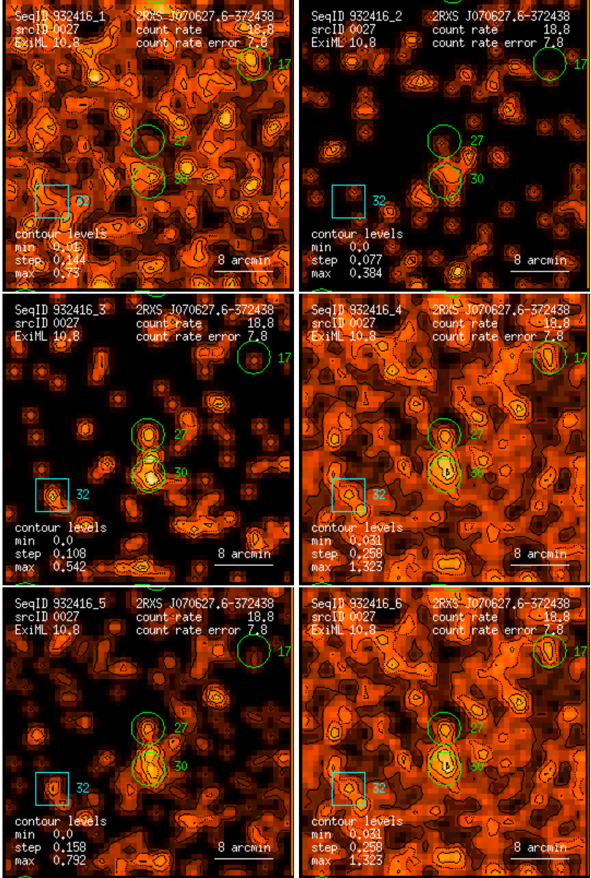
Figure 27: RASS 932416: detection 0027: band rate images, Gaussian filter: (1) PSPC channels 11 – 41, (2) 52 – 90, (3) 91 – 201, (4) 11 – 235, (5) 52 – 201, (6) 11 – 201. Broad band rates in counts/ks. Band rate contour levels in counts/ks/arcmin 2 .
