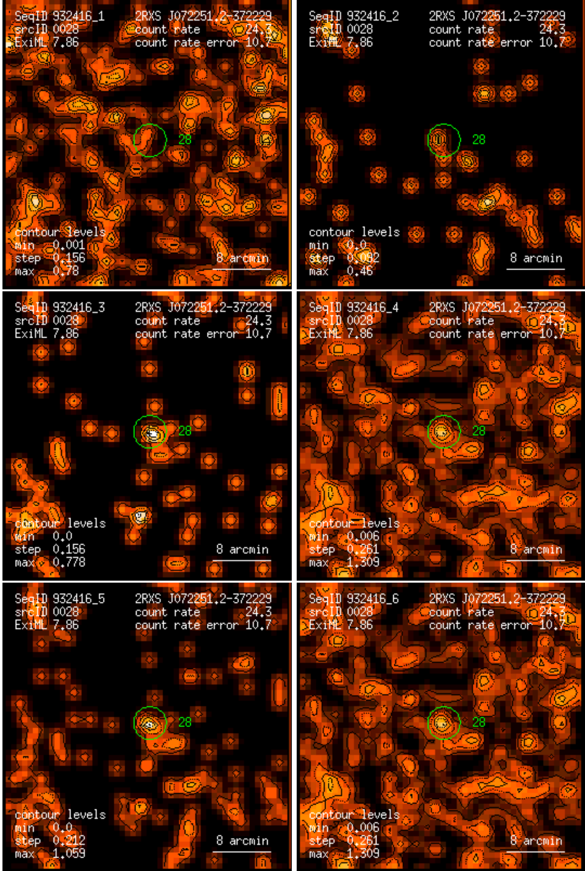
Figure 28: RASS 932416: detection 0028: band rate images, Gaussian filter: (1) PSPC channels 11 – 41, (2) 52 – 90, (3) 91 – 201, (4) 11 – 235, (5) 52 – 201, (6) 11 – 201. Broad band rates in counts/ks. Band rate contour levels in counts/ks/arcmin 2 .
