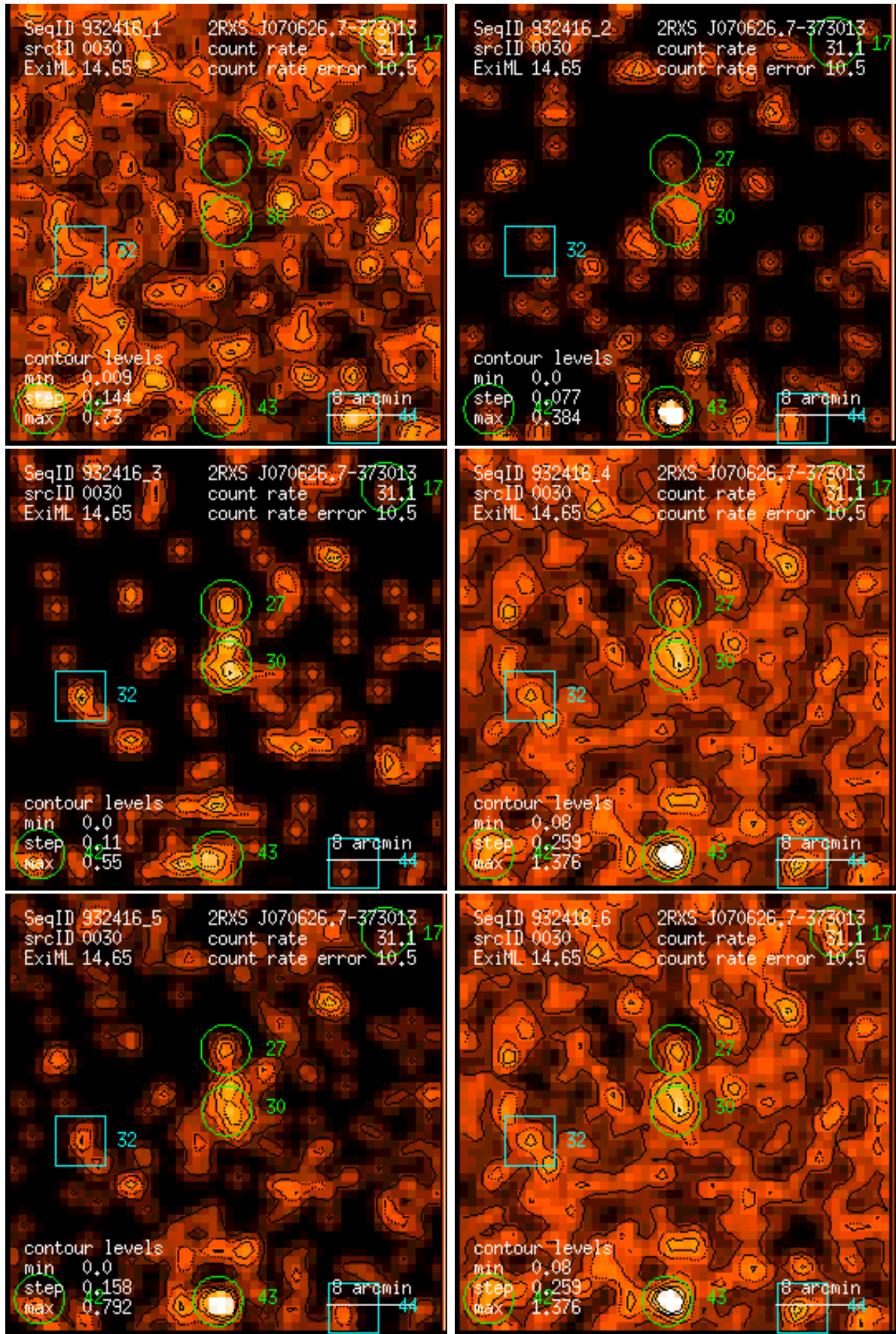
Figure 30: RASS 932416: detection 0030: band rate images, Gaussian filter: (1) PSPC channels 11 – 41, (2) 52 – 90, (3) 91 – 201, (4) 11 – 235, (5) 52 – 201, (6) 11 – 201. Broad band rates in counts/ks. Band rate contour levels in counts/ks/arcmin 2 .
