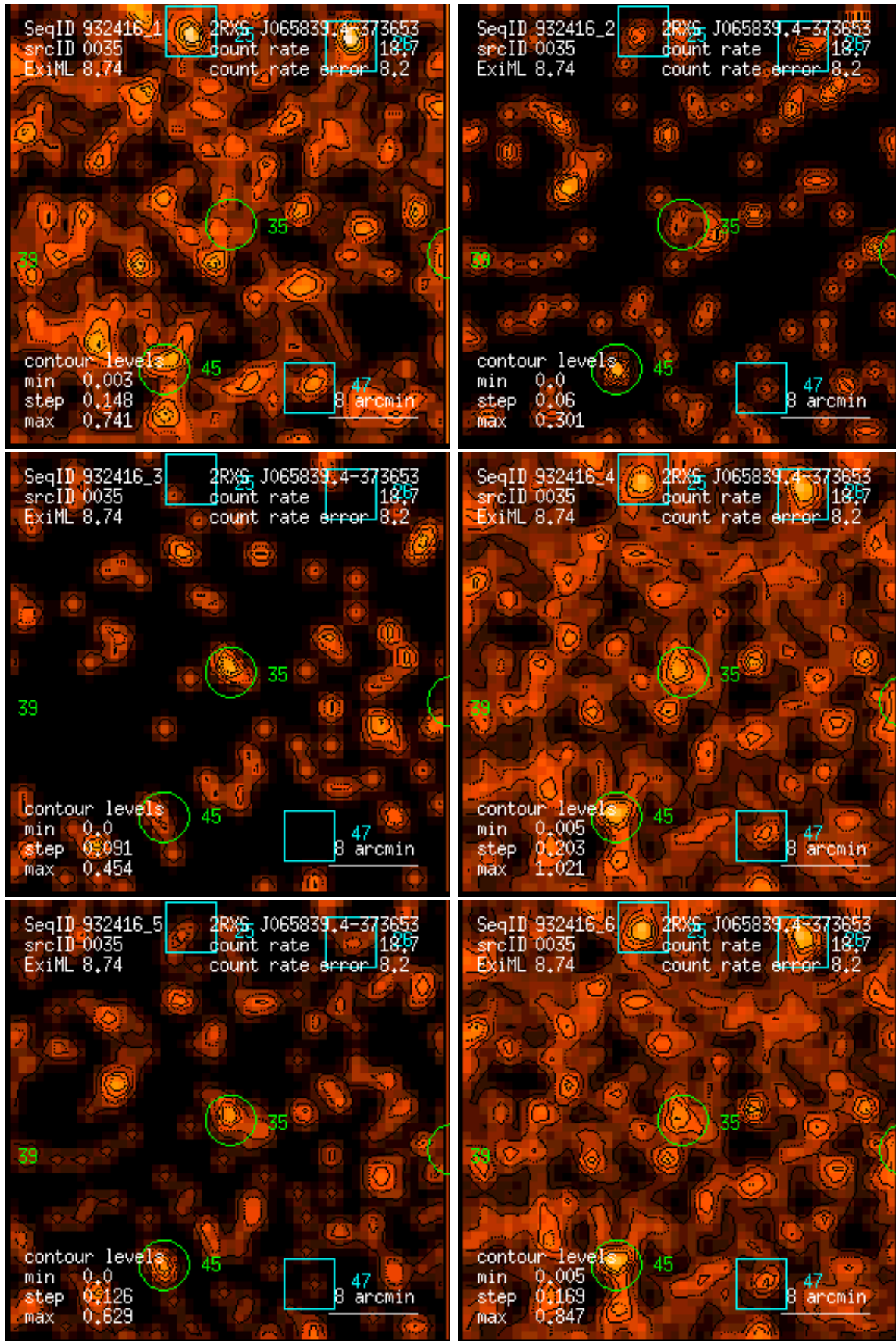
Figure 35: RASS 932416: detection 0035: band rate images, Gaussian filter: (1) PSPC channels 11 – 41, (2) 52 – 90, (3) 91 – 201, (4) 11 – 235, (5) 52 – 201, (6) 11 – 201. Broad band rates in counts/ks. Band rate contour levels in counts/ks/arcmin 2 .
