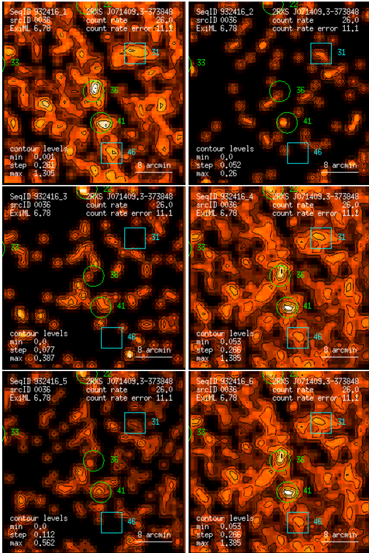
Figure 36: RASS 932416: detection 0036: band rate images, Gaussian filter: (1) PSPC channels 11 – 41, (2) 52 – 90, (3) 91 – 201, (4) 11 – 235, (5) 52 – 201, (6) 11 – 201. Broad band rates in counts/ks. Band rate contour levels in counts/ks/arcmin 2 .
