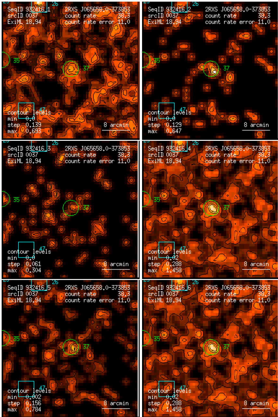
Figure 37: RASS 932416: detection 0037: band rate images, Gaussian filter: (1) PSPC channels 11 – 41, (2) 52 – 90, (3) 91 – 201, (4) 11 – 235, (5) 52 – 201, (6) 11 – 201. Broad band rates in counts/ks. Band rate contour levels in counts/ks/arcmin 2 .
