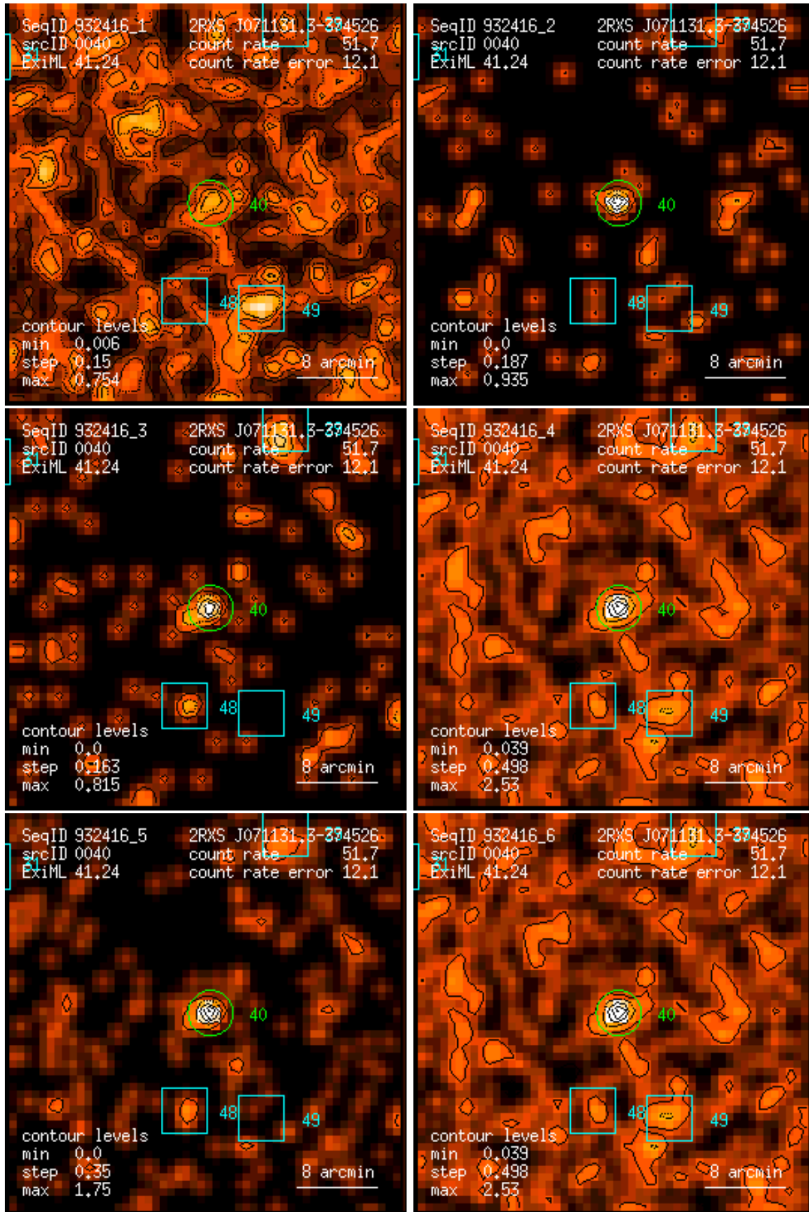
Figure 40: RASS 932416: detection 0040: band rate images, Gaussian filter: (1) PSPC channels 11 – 41, (2) 52 – 90, (3) 91 – 201, (4) 11 – 235, (5) 52 – 201, (6) 11 – 201. Broad band rates in counts/ks. Band rate contour levels in counts/ks/arcmin 2 .
