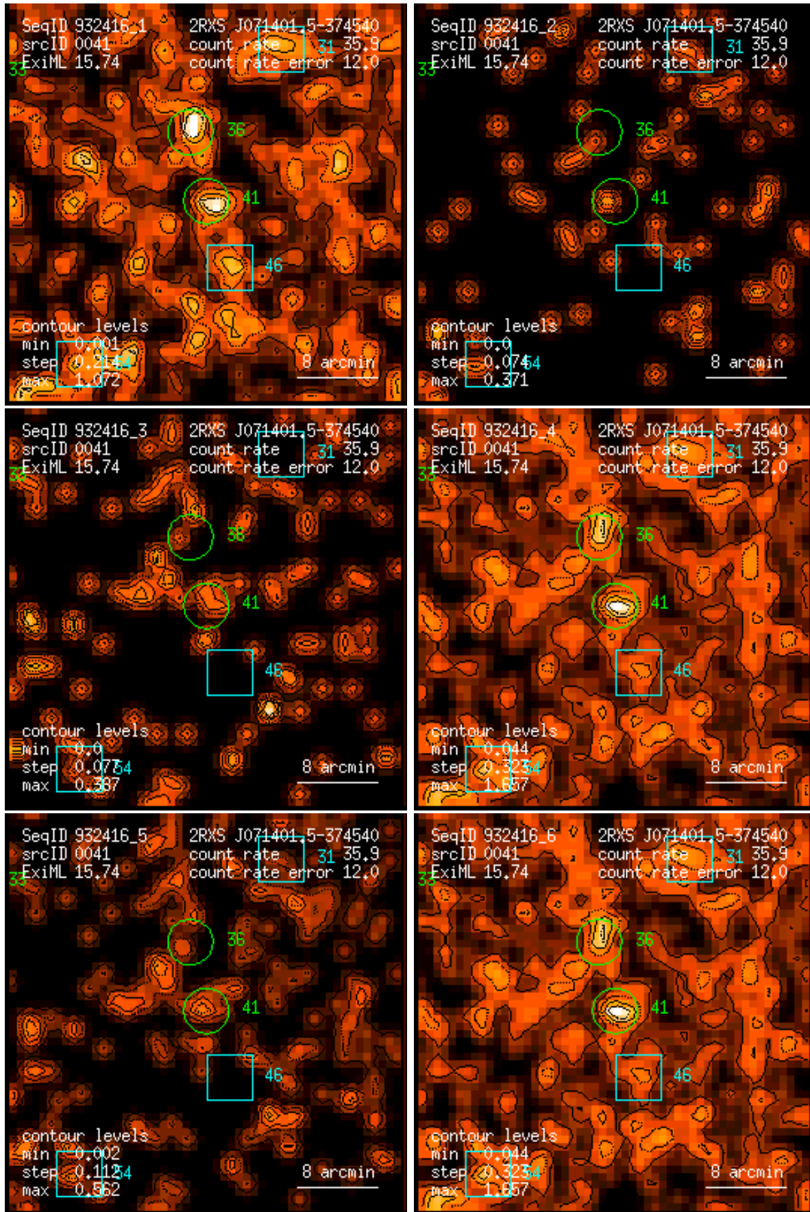
Figure 41: RASS 932416: detection 0041: band rate images, Gaussian filter: (1) PSPC channels 11 – 41, (2) 52 – 90, (3) 91 – 201, (4) 11 – 235, (5) 52 – 201, (6) 11 – 201. Broad band rates in counts/ks. Band rate contour levels in counts/ks/arcmin 2 .
