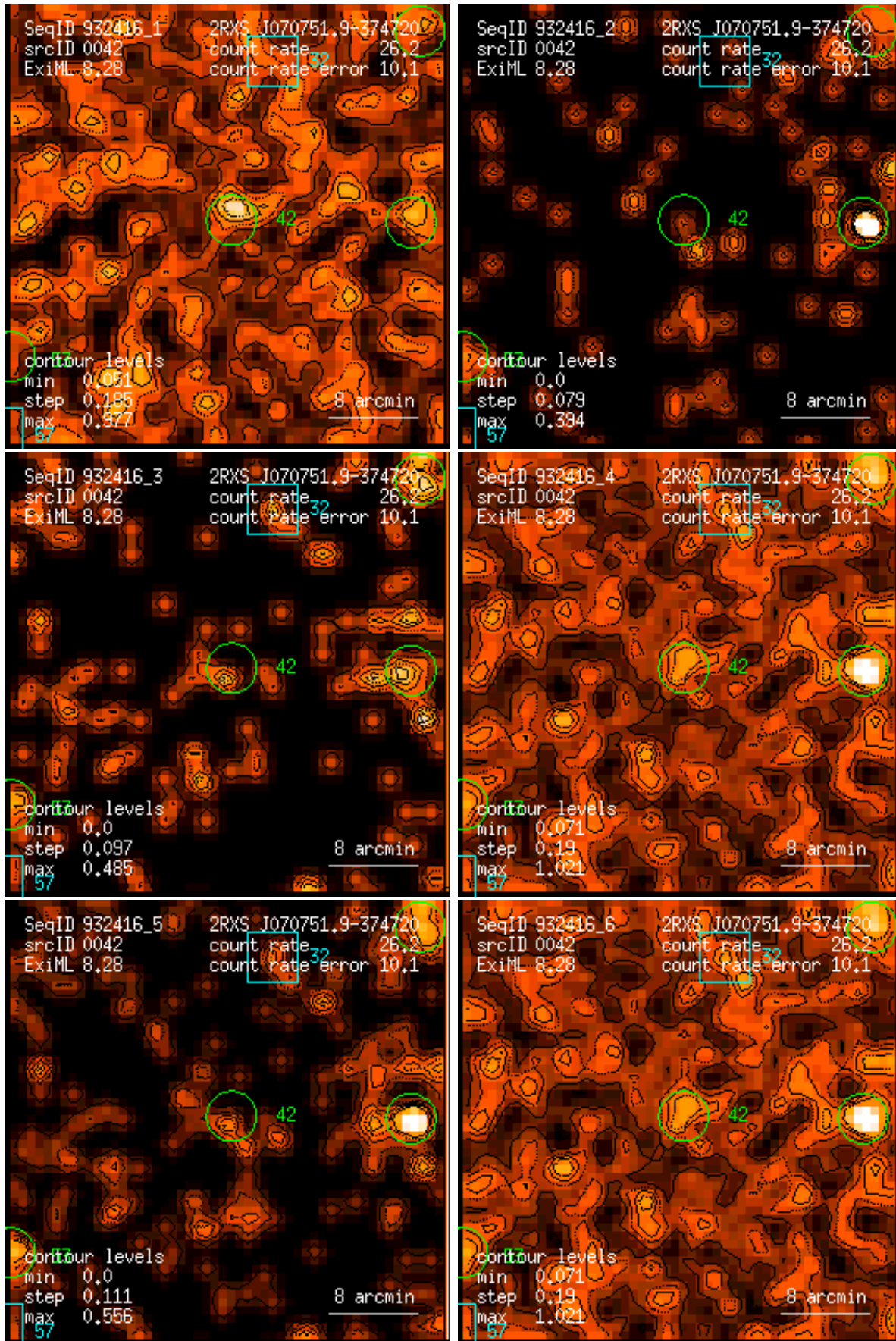
Figure 42: RASS 932416: detection 0042: band rate images, Gaussian filter: (1) PSPC channels 11 – 41, (2) 52 – 90, (3) 91 – 201, (4) 11 – 235, (5) 52 – 201, (6) 11 – 201. Broad band rates in counts/ks. Band rate contour levels in counts/ks/arcmin 2 .
