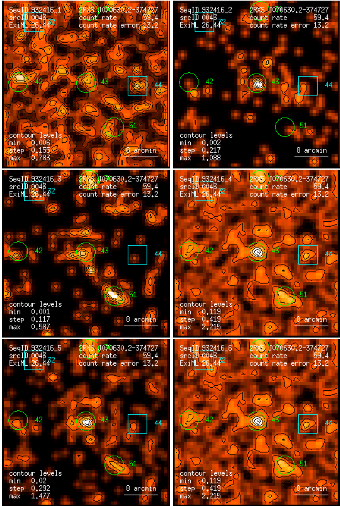
Figure 43: RASS 932416: detection 0043: band rate images, Gaussian filter: (1) PSPC channels 11 – 41, (2) 52 – 90, (3) 91 – 201, (4) 11 – 235, (5) 52 – 201, (6) 11 – 201. Broad band rates in counts/ks. Band rate contour levels in counts/ks/arcmin 2 .
