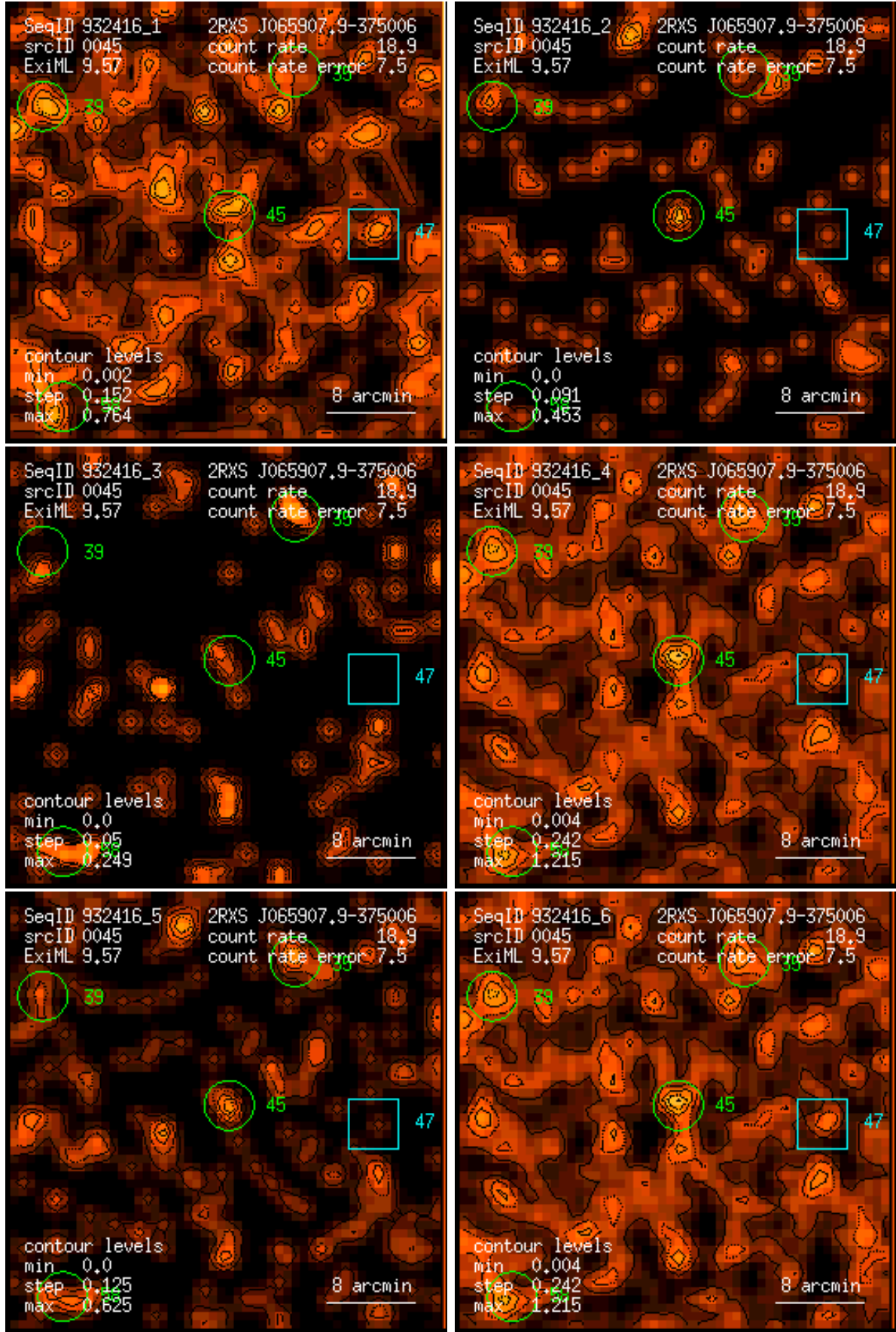
Figure 45: RASS 932416: detection 0045: band rate images, Gaussian filter: (1) PSPC channels 11 – 41, (2) 52 – 90, (3) 91 – 201, (4) 11 – 235, (5) 52 – 201, (6) 11 – 201. Broad band rates in counts/ks. Band rate contour levels in counts/ks/arcmin 2 .
