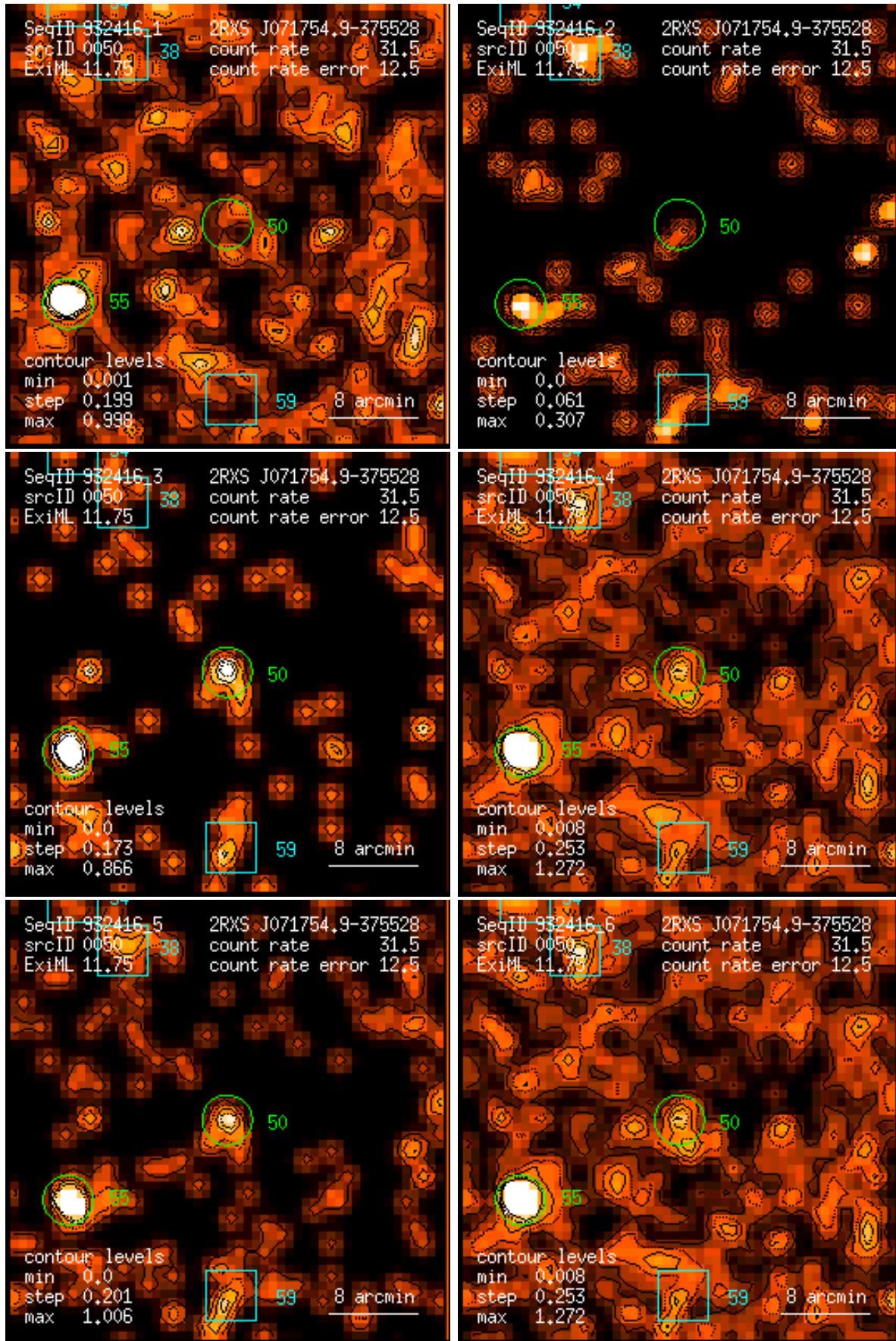
Figure 50: RASS 932416: detection 0050: band rate images, Gaussian filter: (1) PSPC channels 11 – 41, (2) 52 – 90, (3) 91 – 201, (4) 11 – 235, (5) 52 – 201, (6) 11 – 201. Broad band rates in counts/ks. Band rate contour levels in counts/ks/arcmin 2 .
