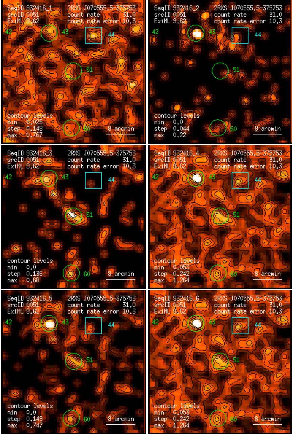
Figure 51: RASS 932416: detection 0051: band rate images, Gaussian filter: (1) PSPC channels 11 – 41, (2) 52 – 90, (3) 91 – 201, (4) 11 – 235, (5) 52 – 201, (6) 11 – 201. Broad band rates in counts/ks. Band rate contour levels in counts/ks/arcmin 2 .
