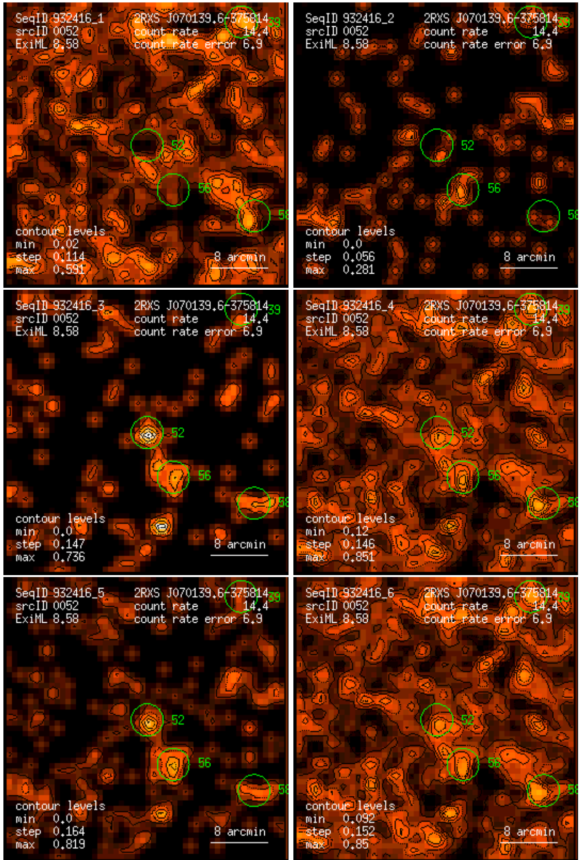
Figure 52: RASS 932416: detection 0052: band rate images, Gaussian filter: (1) PSPC channels 11 – 41, (2) 52 – 90, (3) 91 – 201, (4) 11 – 235, (5) 52 – 201, (6) 11 – 201. Broad band rates in counts/ks. Band rate contour levels in counts/ks/arcmin 2 .
