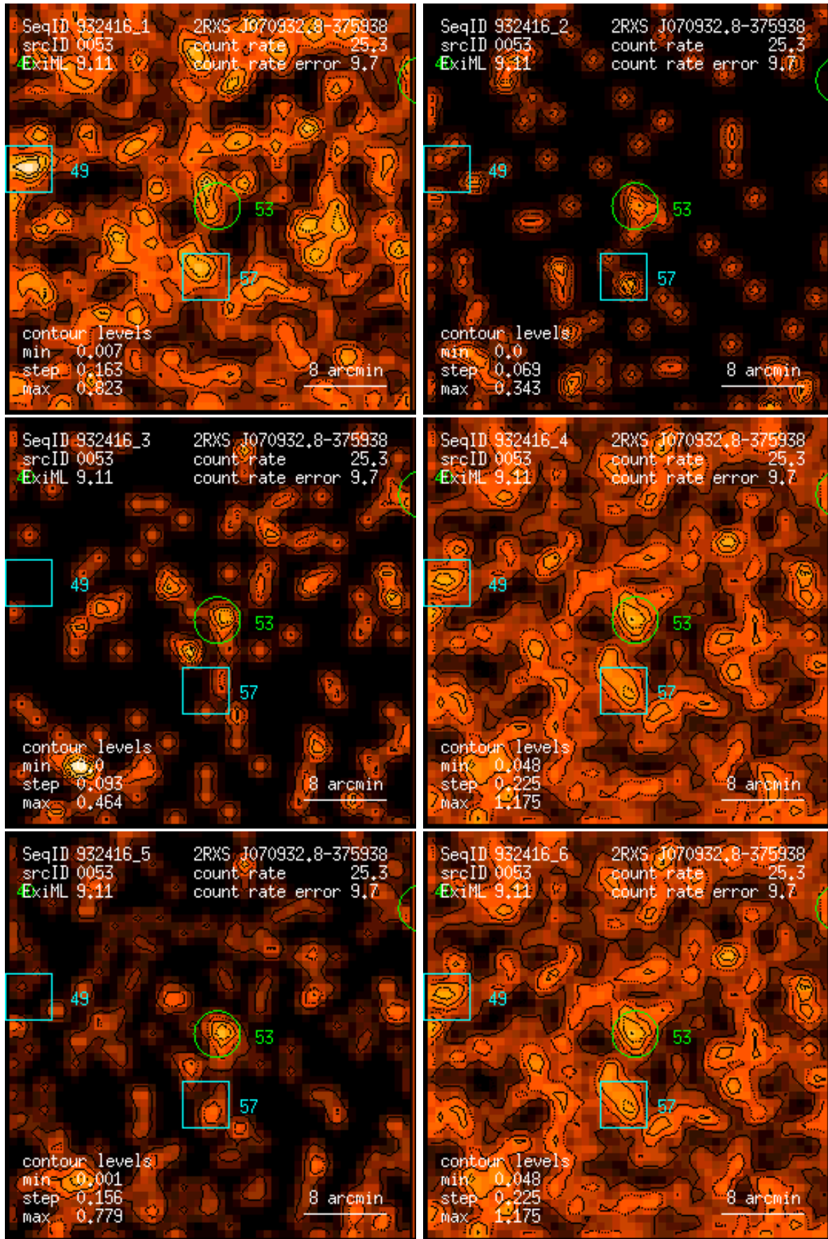
Figure 53: RASS 932416: detection 0053: band rate images, Gaussian filter: (1) PSPC channels 11 – 41, (2) 52 – 90, (3) 91 – 201, (4) 11 – 235, (5) 52 – 201, (6) 11 – 201. Broad band rates in counts/ks. Band rate contour levels in counts/ks/arcmin 2 .
