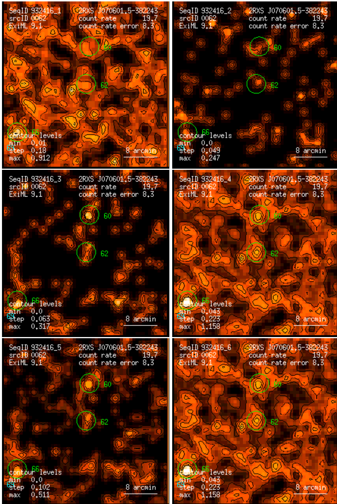
Figure 62: RASS 932416: detection 0062: band rate images, Gaussian filter: (1) PSPC channels 11 – 41, (2) 52 – 90, (3) 91 – 201, (4) 11 – 235, (5) 52 – 201, (6) 11 – 201. Broad band rates in counts/ks. Band rate contour levels in counts/ks/arcmin 2 .
