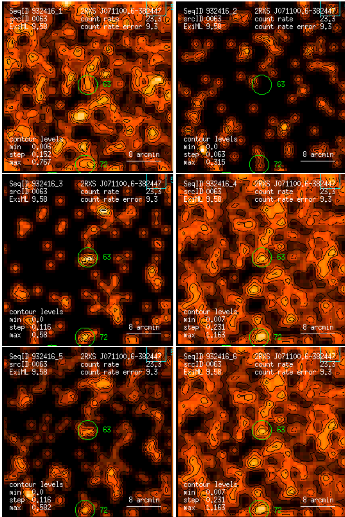
Figure 63: RASS 932416: detection 0063: band rate images, Gaussian filter: (1) PSPC channels 11 – 41, (2) 52 – 90, (3) 91 – 201, (4) 11 – 235, (5) 52 – 201, (6) 11 – 201. Broad band rates in counts/ks. Band rate contour levels in counts/ks/arcmin 2 .
