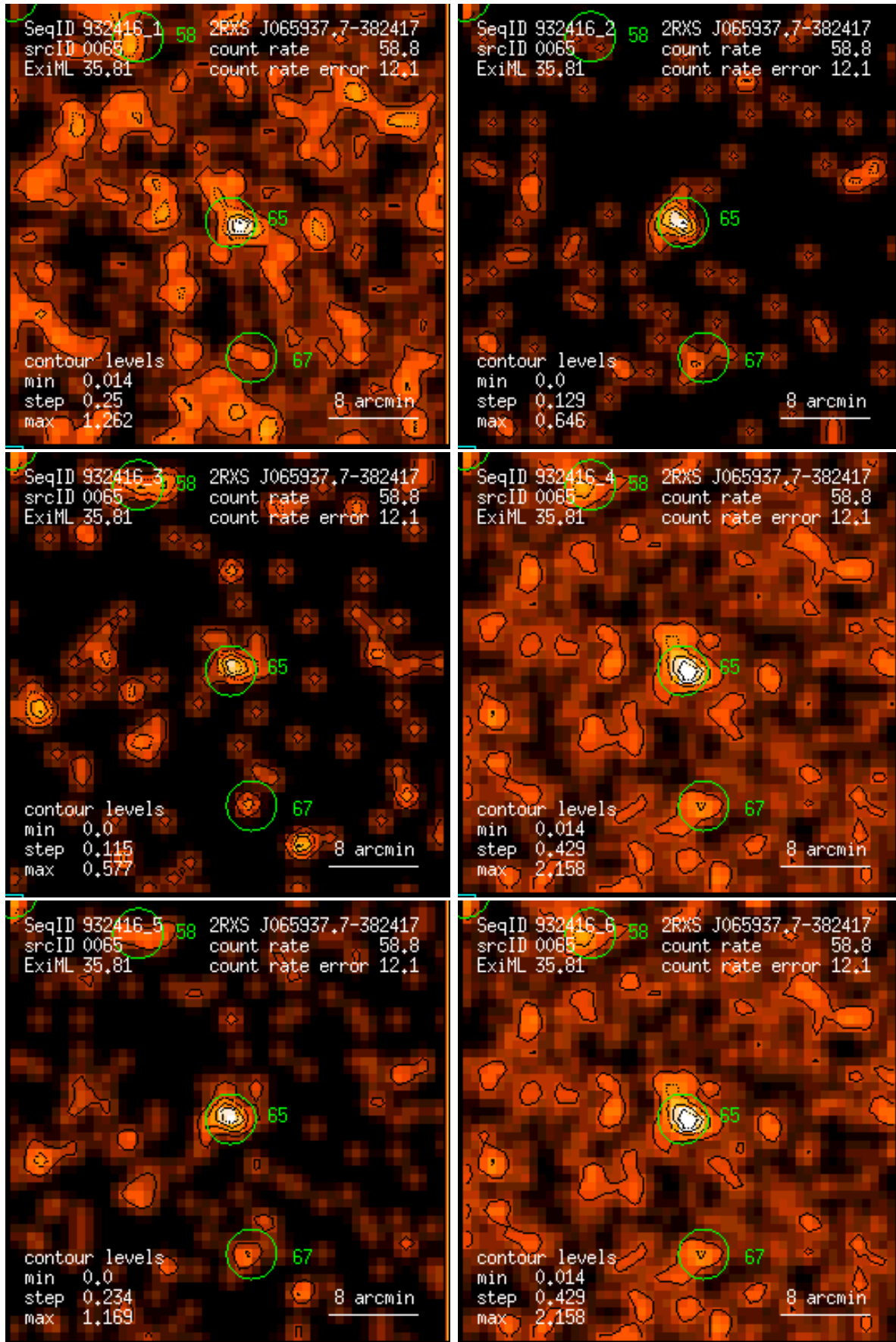
Figure 65: RASS 932416: detection 0065: band rate images, Gaussian filter: (1) PSPC channels 11 – 41, (2) 52 – 90, (3) 91 – 201, (4) 11 – 235, (5) 52 – 201, (6) 11 – 201. Broad band rates in counts/ks. Band rate contour levels in counts/ks/arcmin 2 .
