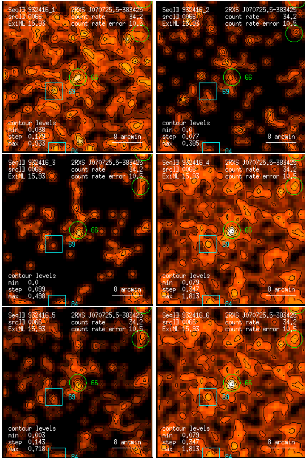
Figure 66: RASS 932416: detection 0066: band rate images, Gaussian filter: (1) PSPC channels 11 – 41, (2) 52 – 90, (3) 91 – 201, (4) 11 – 235, (5) 52 – 201, (6) 11 – 201. Broad band rates in counts/ks. Band rate contour levels in counts/ks/arcmin 2 .
