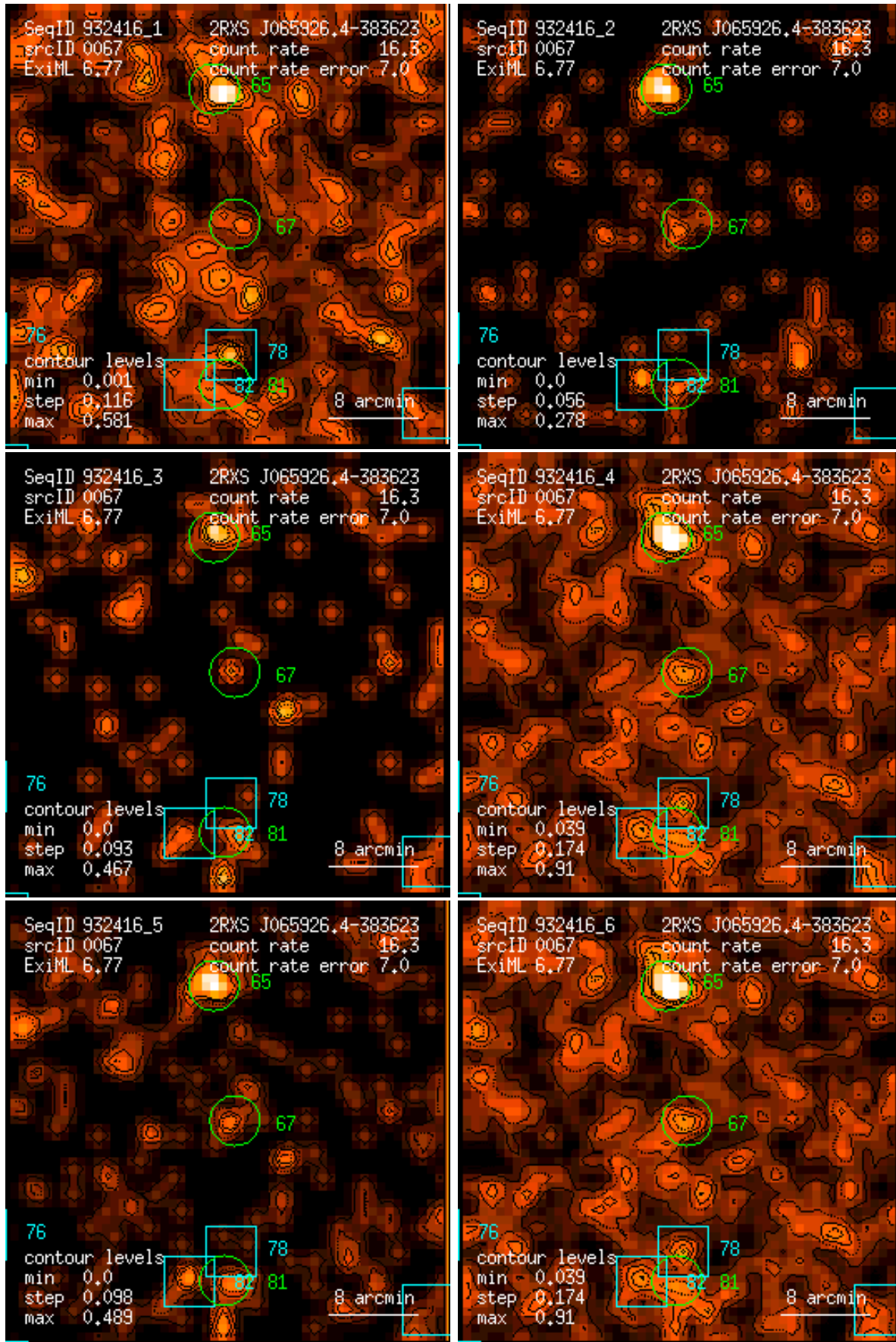
Figure 67: RASS 932416: detection 0067: band rate images, Gaussian filter: (1) PSPC channels 11 – 41, (2) 52 – 90, (3) 91 – 201, (4) 11 – 235, (5) 52 – 201, (6) 11 – 201. Broad band rates in counts/ks. Band rate contour levels in counts/ks/arcmin 2 .
