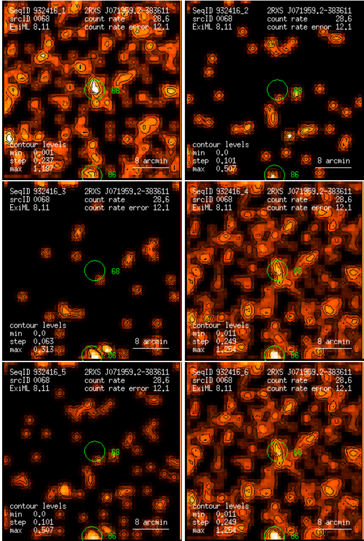
Figure 68: RASS 932416: detection 0068: band rate images, Gaussian filter: (1) PSPC channels 11 – 41, (2) 52 – 90, (3) 91 – 201, (4) 11 – 235, (5) 52 – 201, (6) 11 – 201. Broad band rates in counts/ks. Band rate contour levels in counts/ks/arcmin 2 .
