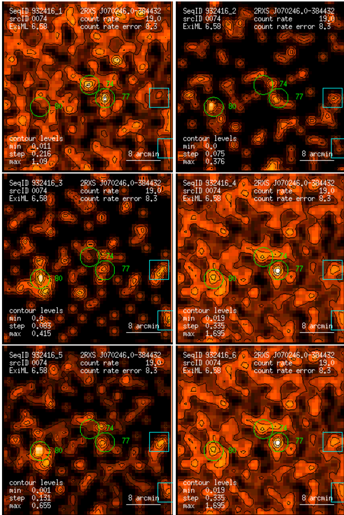
Figure 74: RASS 932416: detection 0074: band rate images, Gaussian filter: (1) PSPC channels 11 – 41, (2) 52 – 90, (3) 91 – 201, (4) 11 – 235, (5) 52 – 201, (6) 11 – 201. Broad band rates in counts/ks. Band rate contour levels in counts/ks/arcmin 2 .
