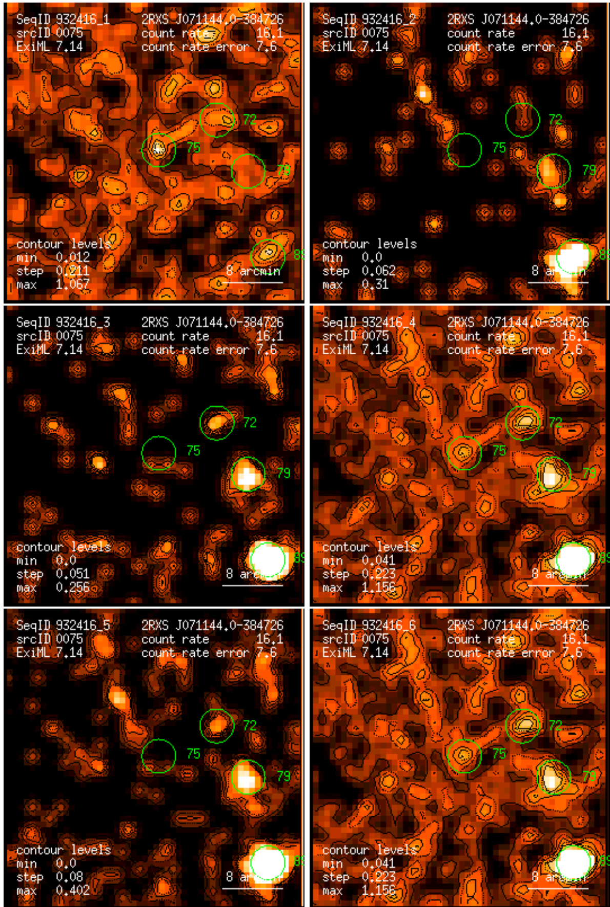
Figure 75: RASS 932416: detection 0075: band rate images, Gaussian filter: (1) PSPC channels 11 – 41, (2) 52 – 90, (3) 91 – 201, (4) 11 – 235, (5) 52 – 201, (6) 11 – 201. Broad band rates in counts/ks. Band rate contour levels in counts/ks/arcmin 2 .
