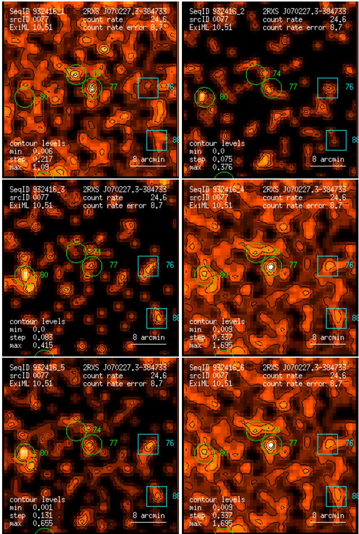
Figure 77: RASS 932416: detection 0077: band rate images, Gaussian filter: (1) PSPC channels 11 – 41, (2) 52 – 90, (3) 91 – 201, (4) 11 – 235, (5) 52 – 201, (6) 11 – 201. Broad band rates in counts/ks. Band rate contour levels in counts/ks/arcmin 2 .
