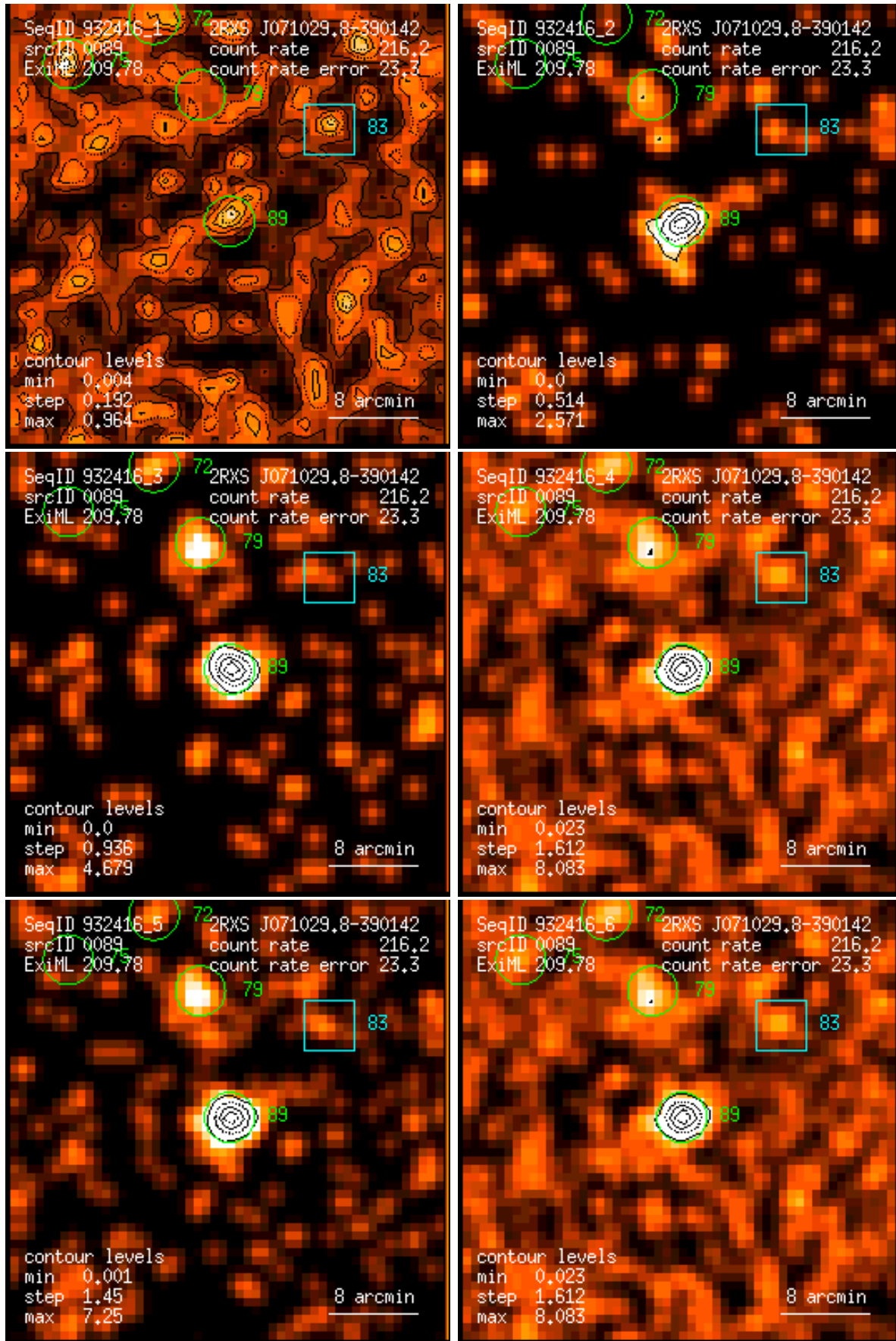
Figure 89: RASS 932416: detection 0089: band rate images, Gaussian filter: (1) PSPC channels 11 – 41, (2) 52 – 90, (3) 91 – 201, (4) 11 – 235, (5) 52 – 201, (6) 11 – 201. Broad band rates in counts/ks. Band rate contour levels in counts/ks/arcmin 2 .
