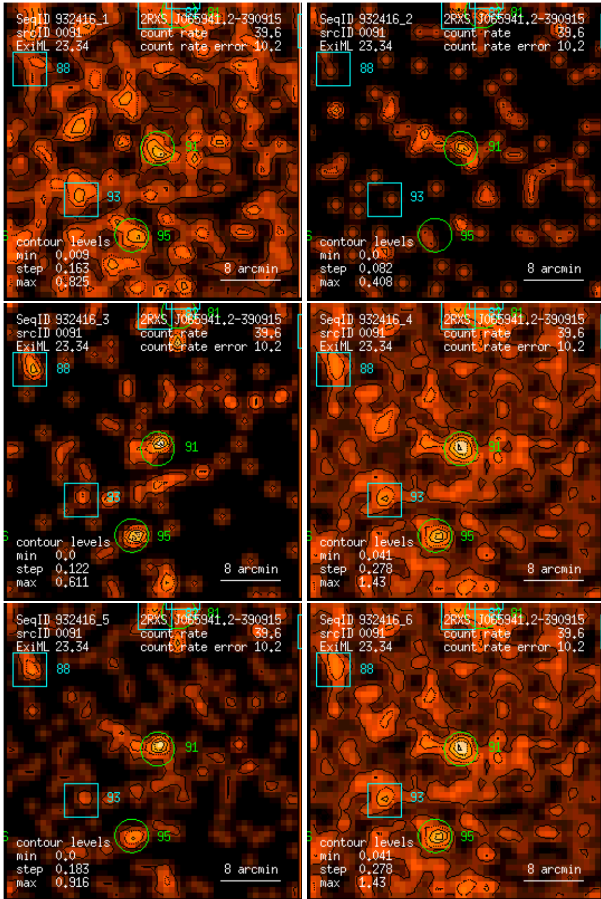
Figure 91: RASS 932416: detection 0091: band rate images, Gaussian filter: (1) PSPC channels 11 – 41, (2) 52 – 90, (3) 91 – 201, (4) 11 – 235, (5) 52 – 201, (6) 11 – 201. Broad band rates in counts/ks. Band rate contour levels in counts/ks/arcmin 2 .
