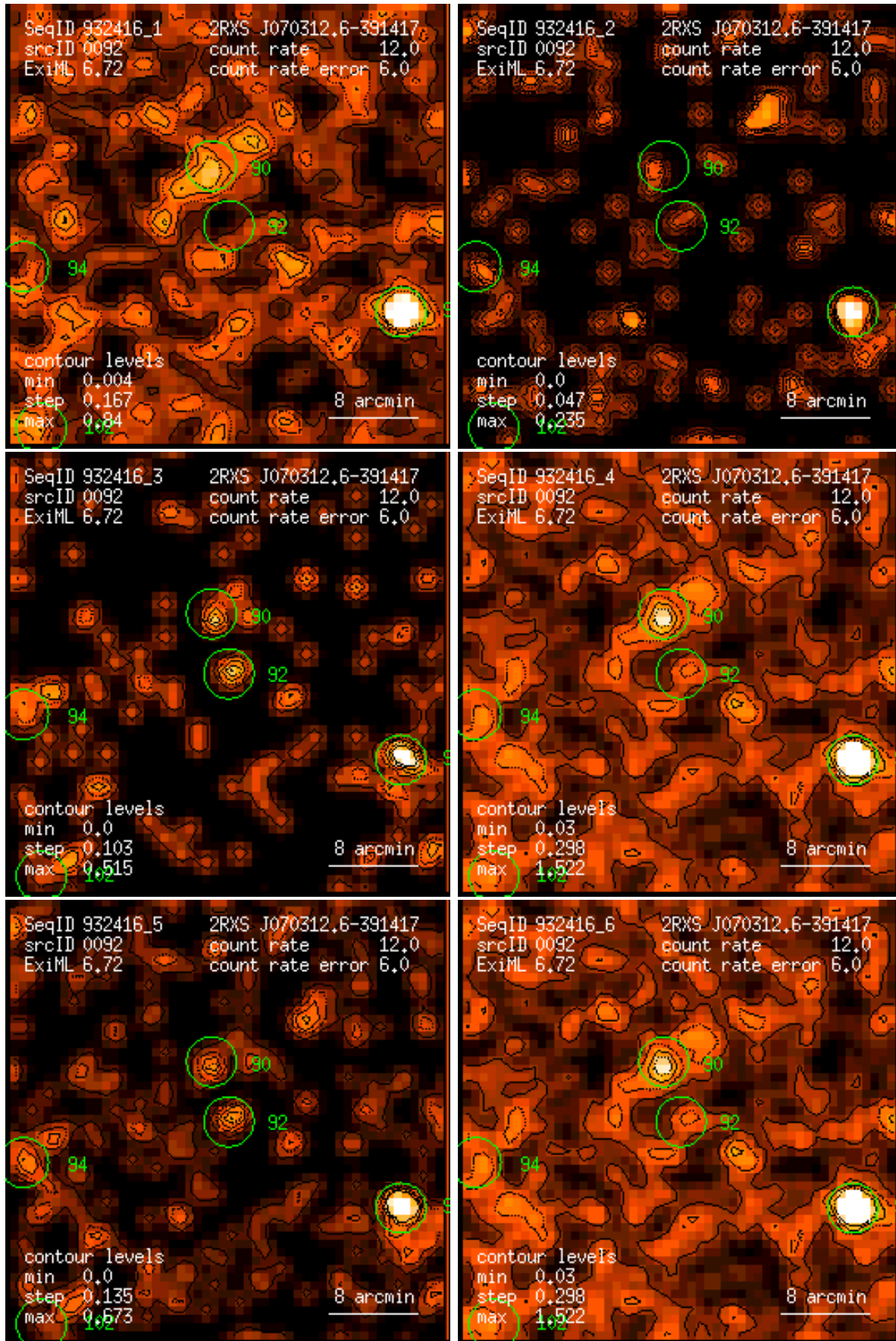
Figure 92: RASS 932416: detection 0092: band rate images, Gaussian filter: (1) PSPC channels 11 – 41, (2) 52 – 90, (3) 91 – 201, (4) 11 – 235, (5) 52 – 201, (6) 11 – 201. Broad band rates in counts/ks. Band rate contour levels in counts/ks/arcmin 2 .
