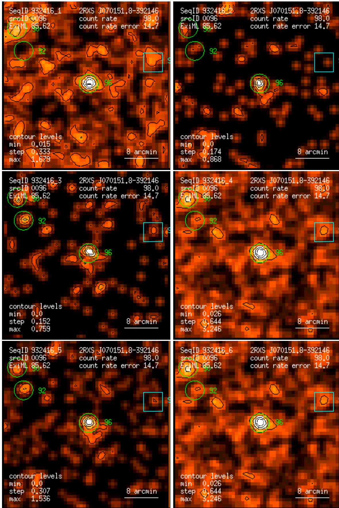
Figure 96: RASS 932416: detection 0096: band rate images, Gaussian filter: (1) PSPC channels 11 – 41, (2) 52 – 90, (3) 91 – 201, (4) 11 – 235, (5) 52 – 201, (6) 11 – 201. Broad band rates in counts/ks. Band rate contour levels in counts/ks/arcmin 2 .
