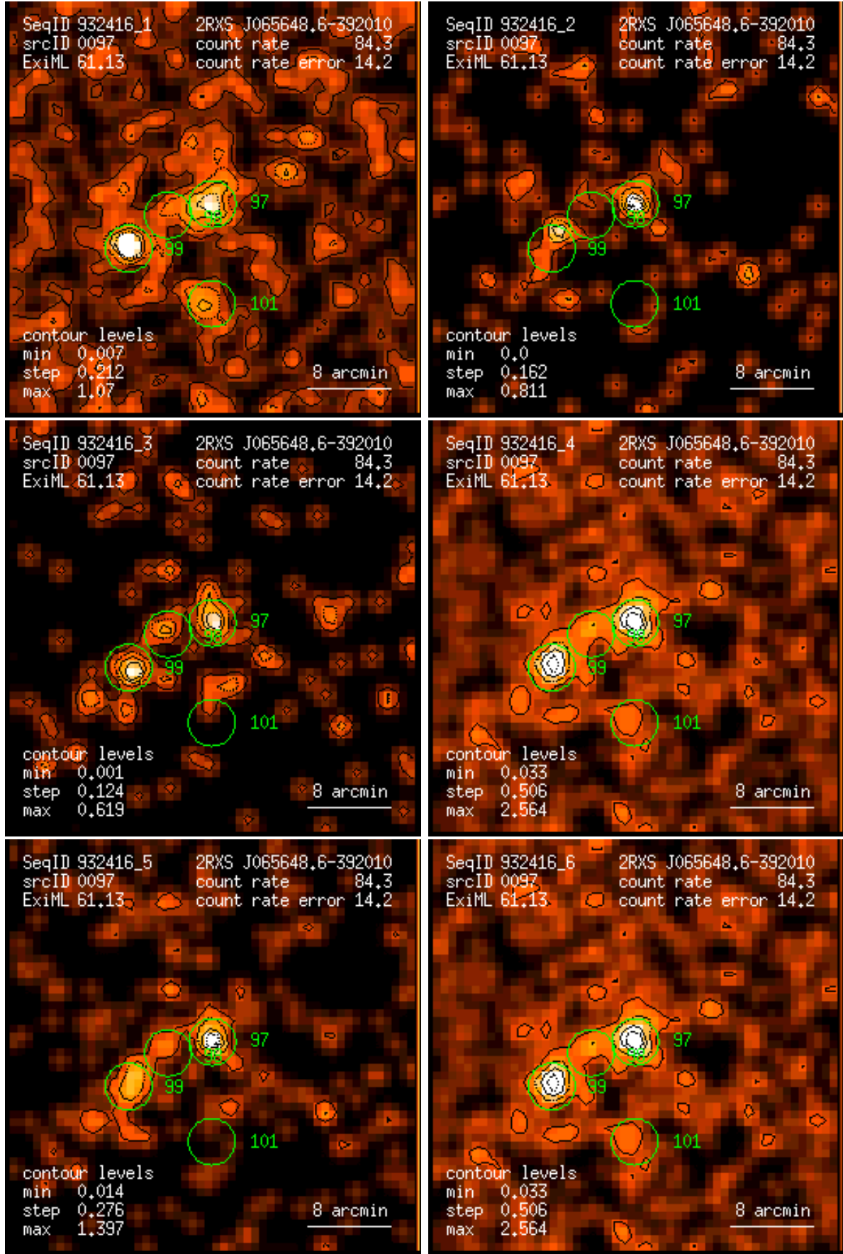
Figure 97: RASS 932416: detection 0097: band rate images, Gaussian filter: (1) PSPC channels 11 – 41, (2) 52 – 90, (3) 91 – 201, (4) 11 – 235, (5) 52 – 201, (6) 11 – 201. Broad band rates in counts/ks. Band rate contour levels in counts/ks/arcmin 2 .
