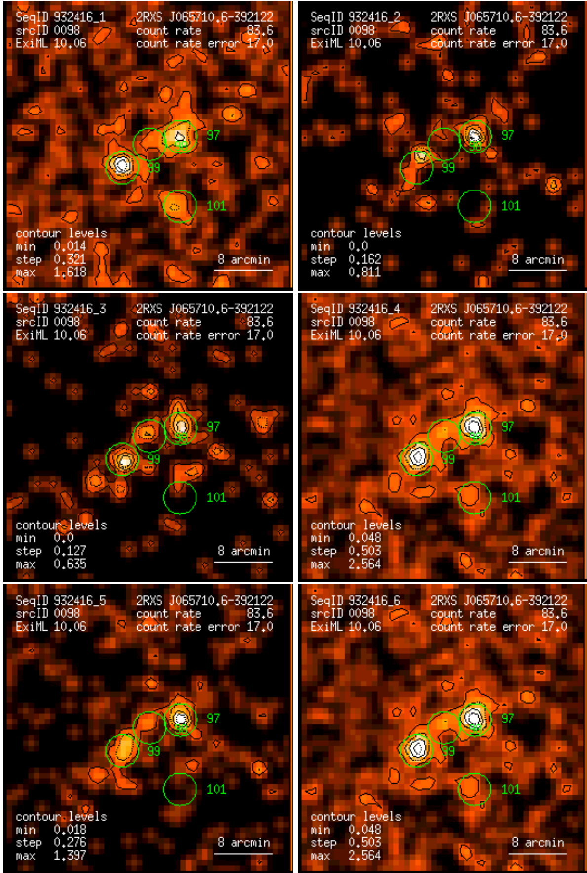
Figure 98: RASS 932416: detection 0098: band rate images, Gaussian filter: (1) PSPC channels 11 – 41, (2) 52 – 90, (3) 91 – 201, (4) 11 – 235, (5) 52 – 201, (6) 11 – 201. Broad band rates in counts/ks. Band rate contour levels in counts/ks/arcmin 2 .
