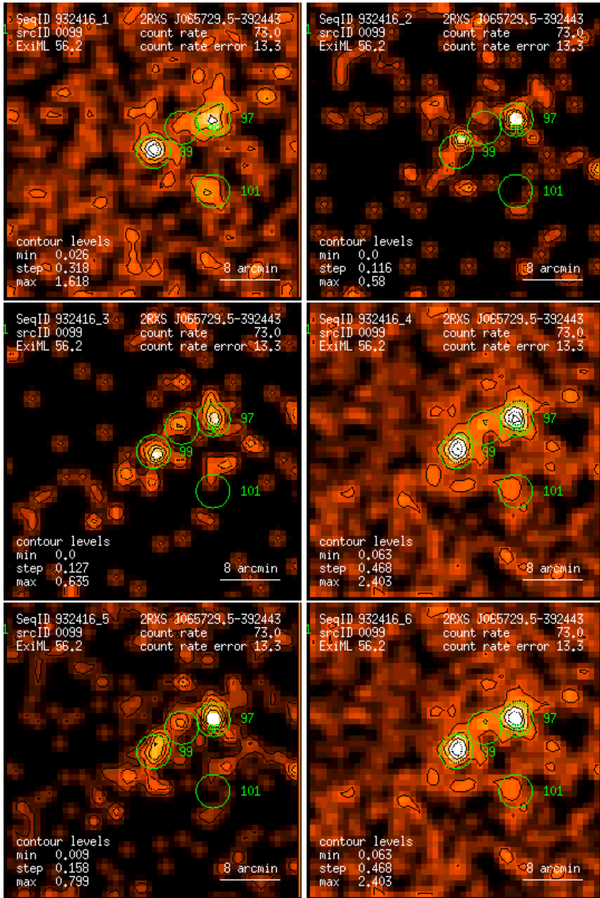
Figure 99: RASS 932416: detection 0099: band rate images, Gaussian filter: (1) PSPC channels 11 – 41, (2) 52 – 90, (3) 91 – 201, (4) 11 – 235, (5) 52 – 201, (6) 11 – 201. Broad band rates in counts/ks. Band rate contour levels in counts/ks/arcmin 2 .
