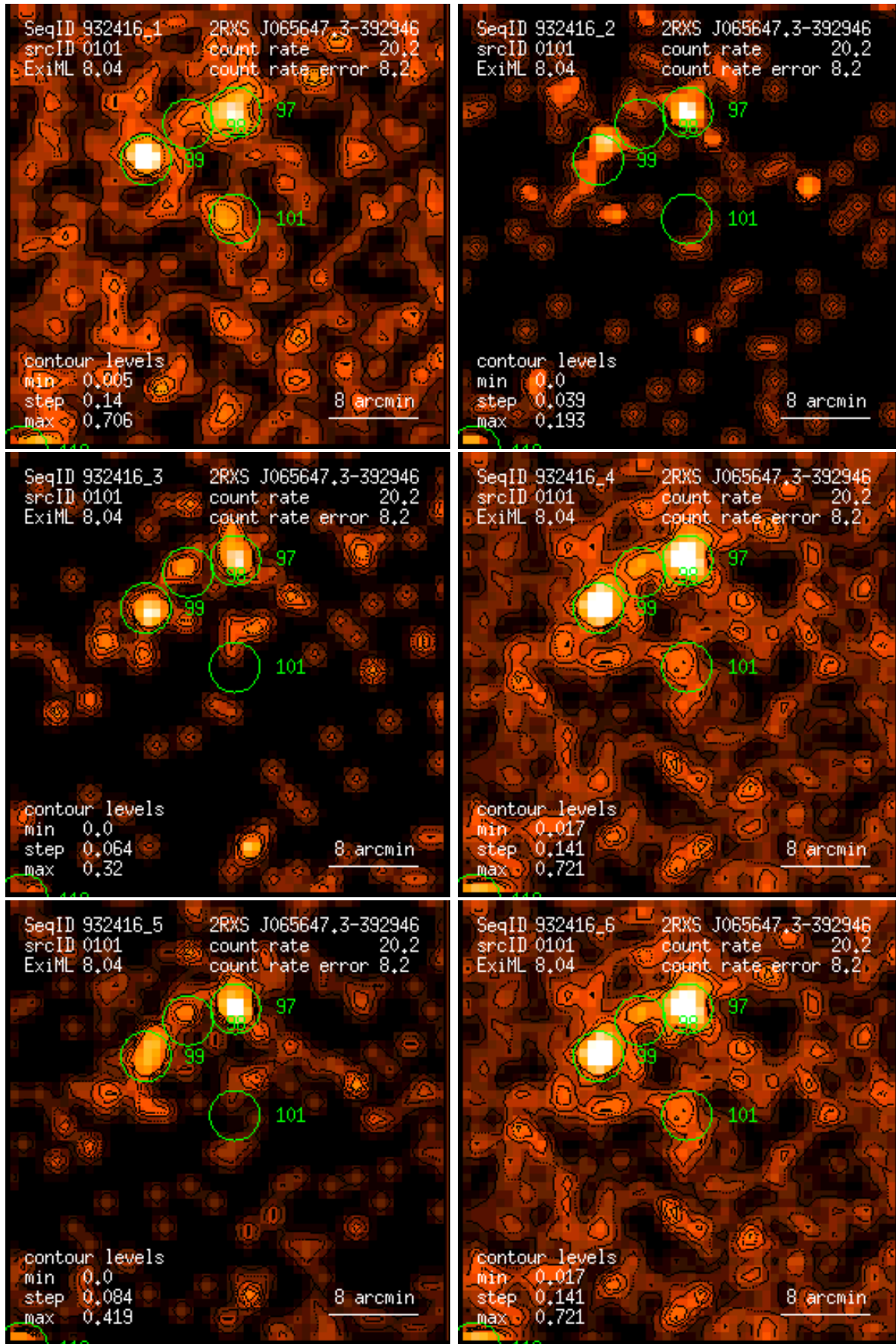
Figure 101: RASS 932416: detection 0101: band rate images, Gaussian filter: (1) PSPC channels 11 – 41, (2) 52 – 90, (3) 91 – 201, (4) 11 – 235, (5) 52 – 201, (6) 11 – 201. Broad band rates in counts/ks. Band rate contour levels in counts/ks/arcmin 2 .
