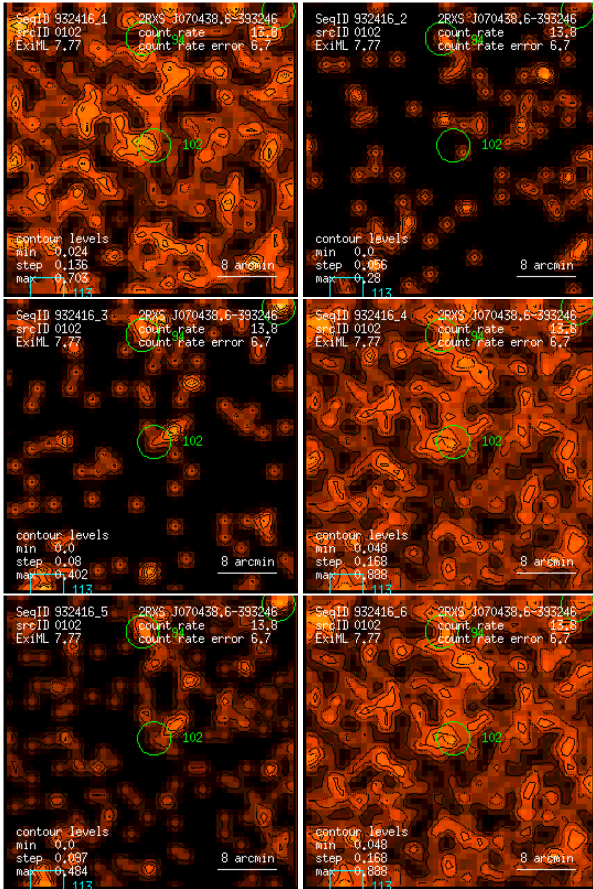
Figure 102: RASS 932416: detection 0102: band rate images, Gaussian filter: (1) PSPC channels 11 – 41, (2) 52 – 90, (3) 91 – 201, (4) 11 – 235, (5) 52 – 201, (6) 11 – 201. Broad band rates in counts/ks. Band rate contour levels in counts/ks/arcmin 2 .
