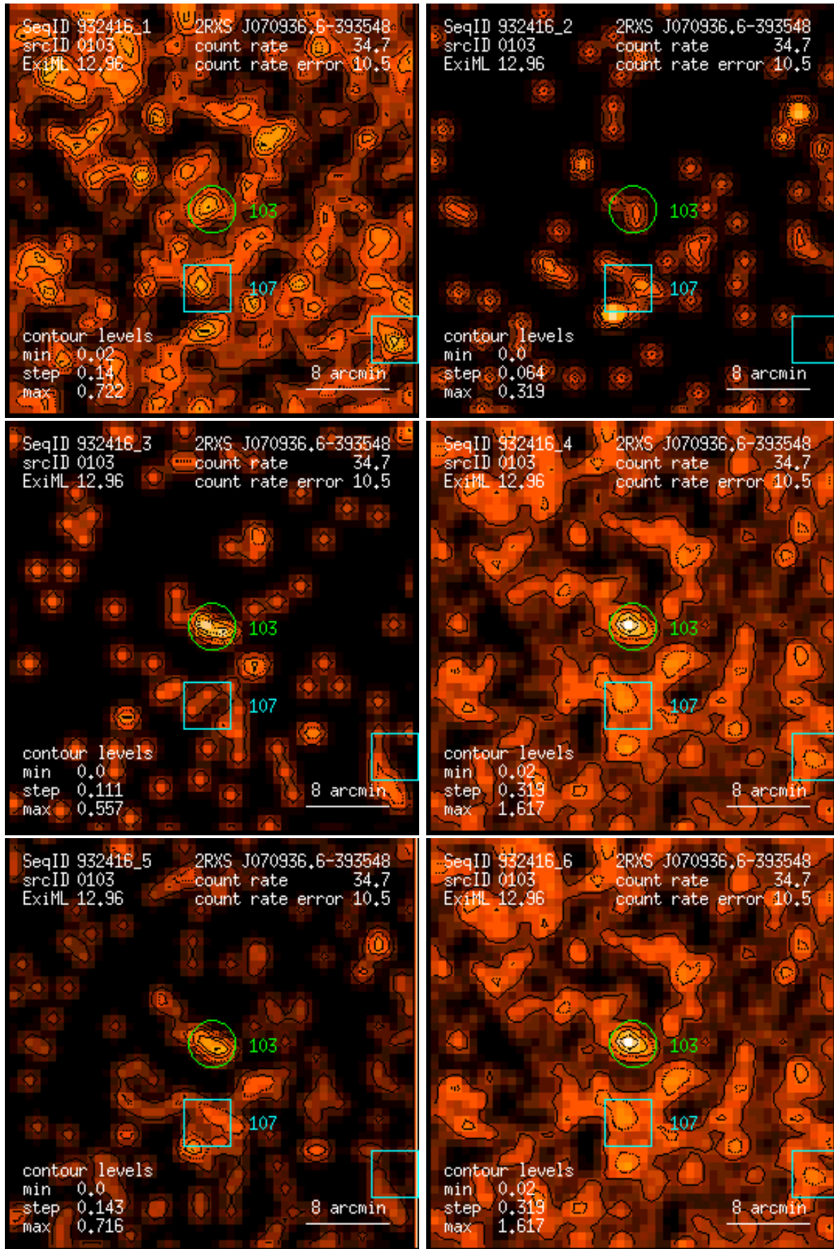
Figure 103: RASS 932416: detection 0103: band rate images, Gaussian filter: (1) PSPC channels 11 – 41, (2) 52 – 90, (3) 91 – 201, (4) 11 – 235, (5) 52 – 201, (6) 11 – 201. Broad band rates in counts/ks. Band rate contour levels in counts/ks/arcmin 2 .
