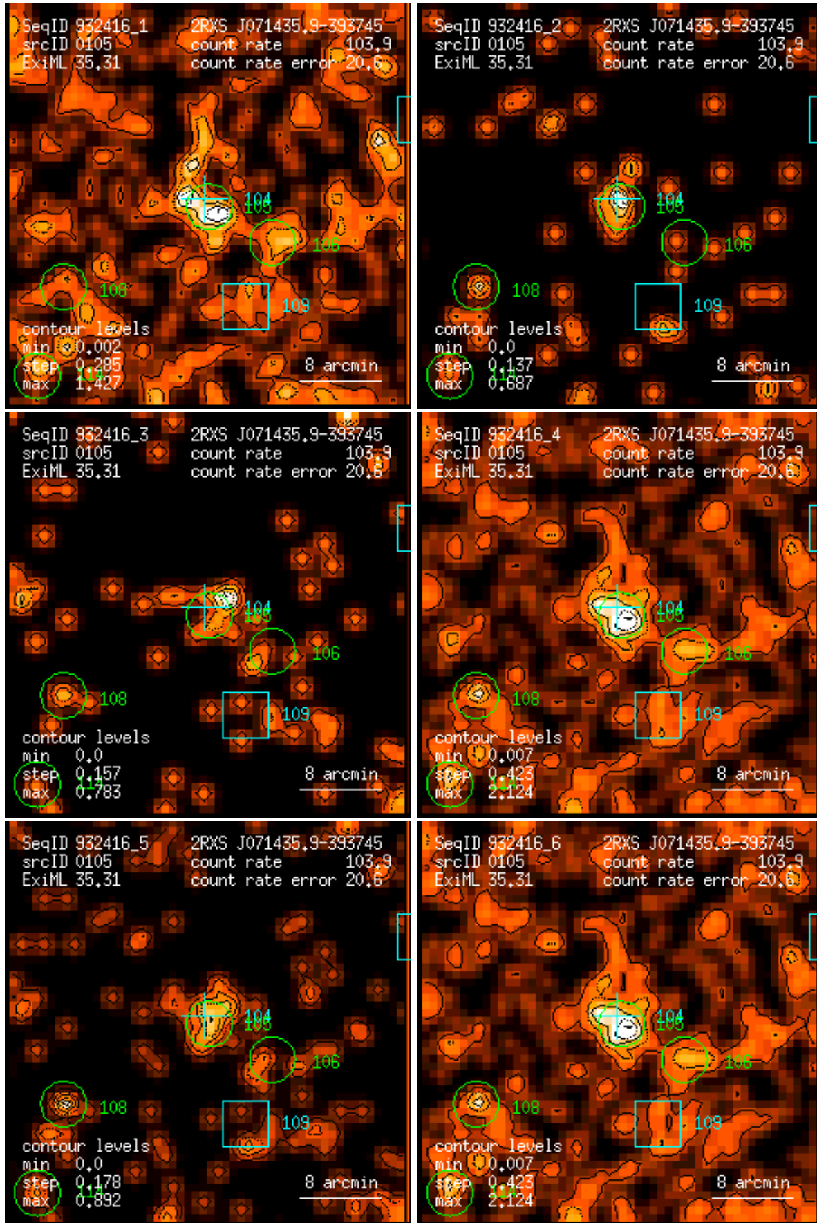
Figure 105: RASS 932416: detection 0105: band rate images, Gaussian filter: (1) PSPC channels 11 – 41, (2) 52 – 90, (3) 91 – 201, (4) 11 – 235, (5) 52 – 201, (6) 11 – 201. Broad band rates in counts/ks. Band rate contour levels in counts/ks/arcmin 2 .
