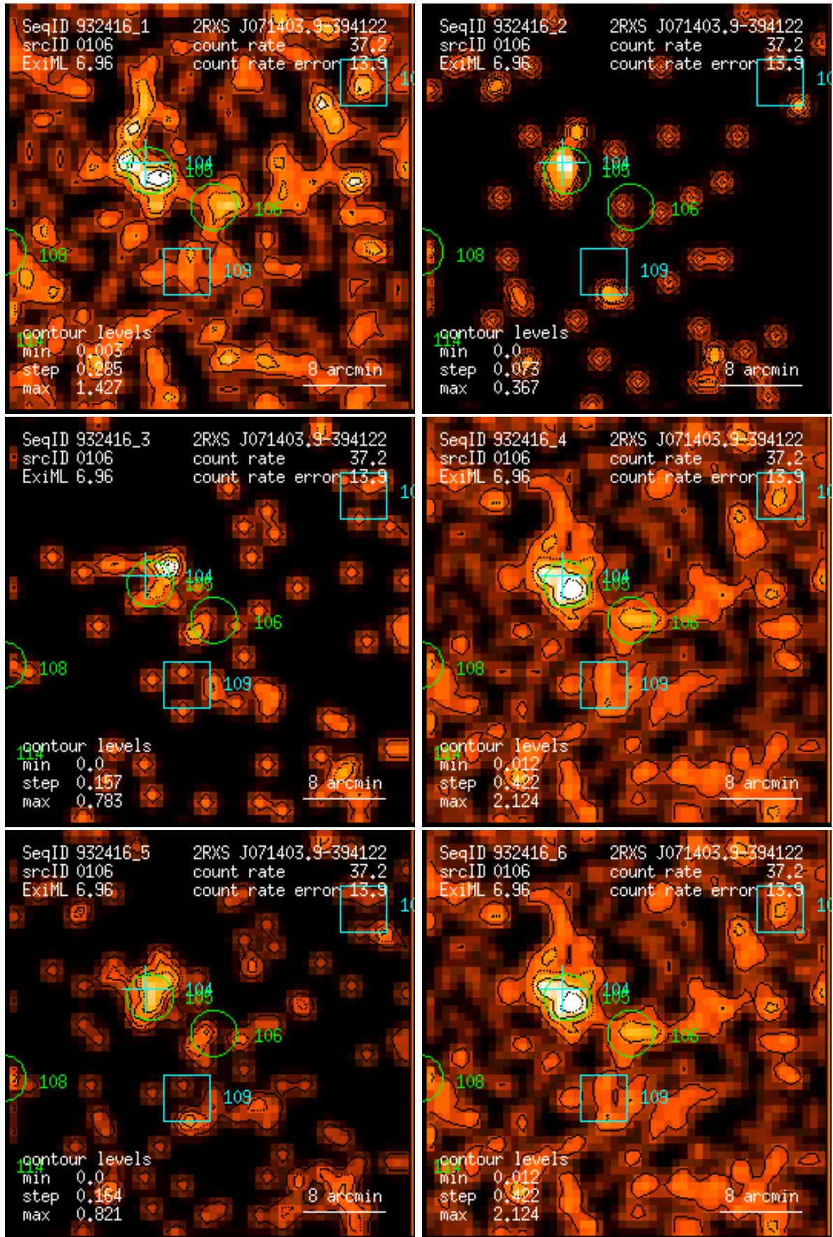
Figure 106: RASS 932416: detection 0106: band rate images, Gaussian filter: (1) PSPC channels 11 – 41, (2) 52 – 90, (3) 91 – 201, (4) 11 – 235, (5) 52 – 201, (6) 11 – 201. Broad band rates in counts/ks. Band rate contour levels in counts/ks/arcmin 2 .
