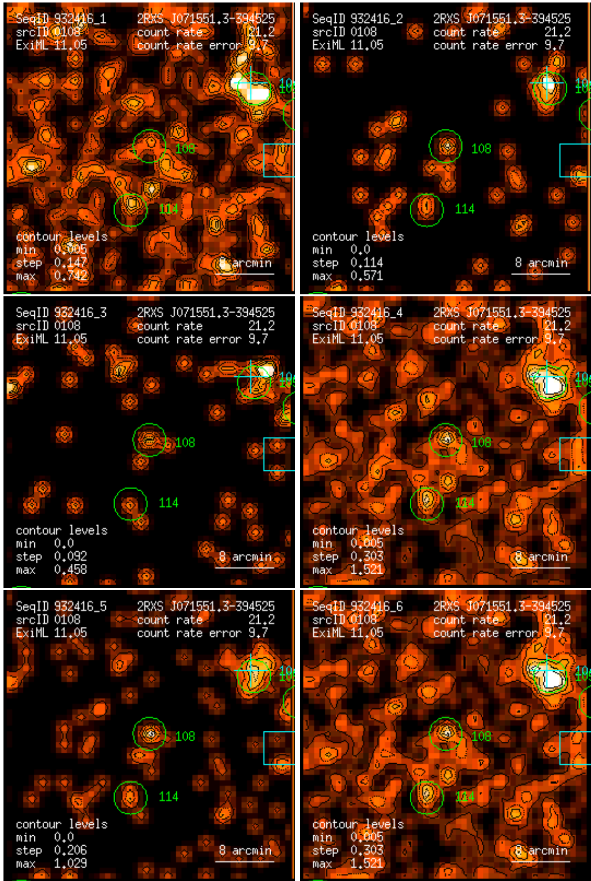
Figure 108: RASS 932416: detection 0108: band rate images, Gaussian filter: (1) PSPC channels 11 – 41, (2) 52 – 90, (3) 91 – 201, (4) 11 – 235, (5) 52 – 201, (6) 11 – 201. Broad band rates in counts/ks. Band rate contour levels in counts/ks/arcmin 2 .
