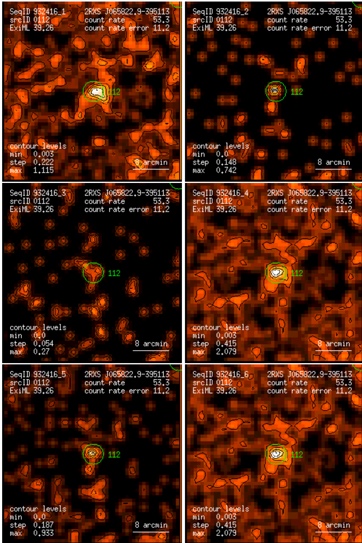
Figure 112: RASS 932416: detection 0112: band rate images, Gaussian filter: (1) PSPC channels 11 – 41, (2) 52 – 90, (3) 91 – 201, (4) 11 – 235, (5) 52 – 201, (6) 11 – 201. Broad band rates in counts/ks. Band rate contour levels in counts/ks/arcmin 2 .
