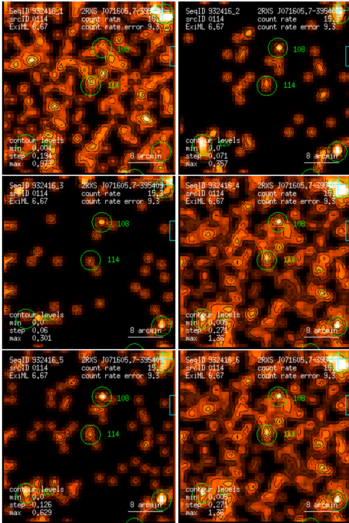
Figure 114: RASS 932416: detection 0114: band rate images, Gaussian filter: (1) PSPC channels 11 – 41, (2) 52 – 90, (3) 91 – 201, (4) 11 – 235, (5) 52 – 201, (6) 11 – 201. Broad band rates in counts/ks. Band rate contour levels in counts/ks/arcmin 2 .
