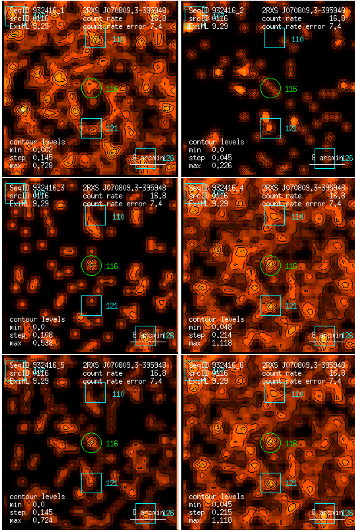
Figure 116: RASS 932416: detection 0116: band rate images, Gaussian filter: (1) PSPC channels 11 – 41, (2) 52 – 90, (3) 91 – 201, (4) 11 – 235, (5) 52 – 201, (6) 11 – 201. Broad band rates in counts/ks. Band rate contour levels in counts/ks/arcmin 2 .
