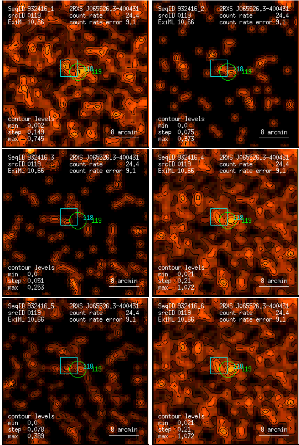
Figure 119: RASS 932416: detection 0119: band rate images, Gaussian filter: (1) PSPC channels 11 – 41, (2) 52 – 90, (3) 91 – 201, (4) 11 – 235, (5) 52 – 201, (6) 11 – 201. Broad band rates in counts/ks. Band rate contour levels in counts/ks/arcmin 2 .
