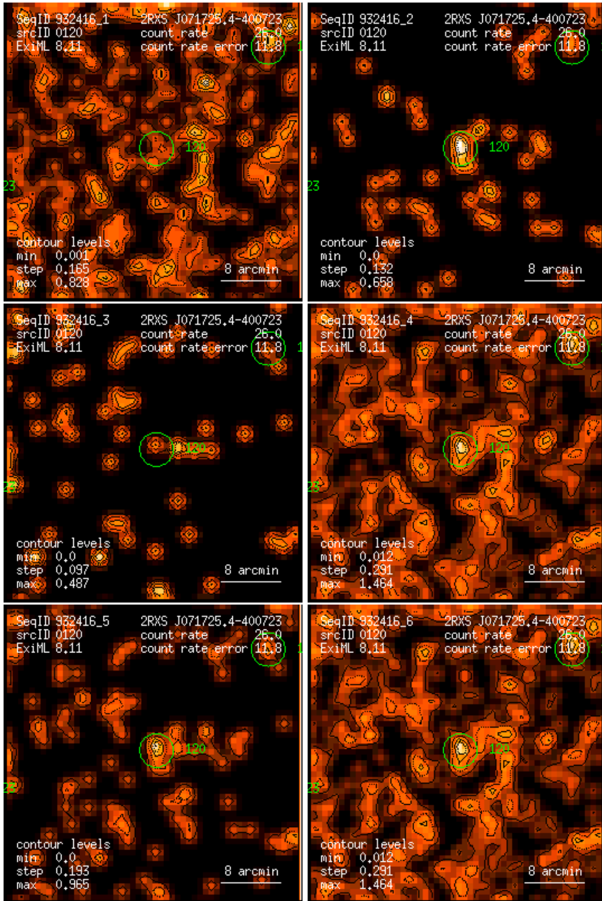
Figure 120: RASS 932416: detection 0120: band rate images, Gaussian filter: (1) PSPC channels 11 – 41, (2) 52 – 90, (3) 91 – 201, (4) 11 – 235, (5) 52 – 201, (6) 11 – 201. Broad band rates in counts/ks. Band rate contour levels in counts/ks/arcmin 2 .
