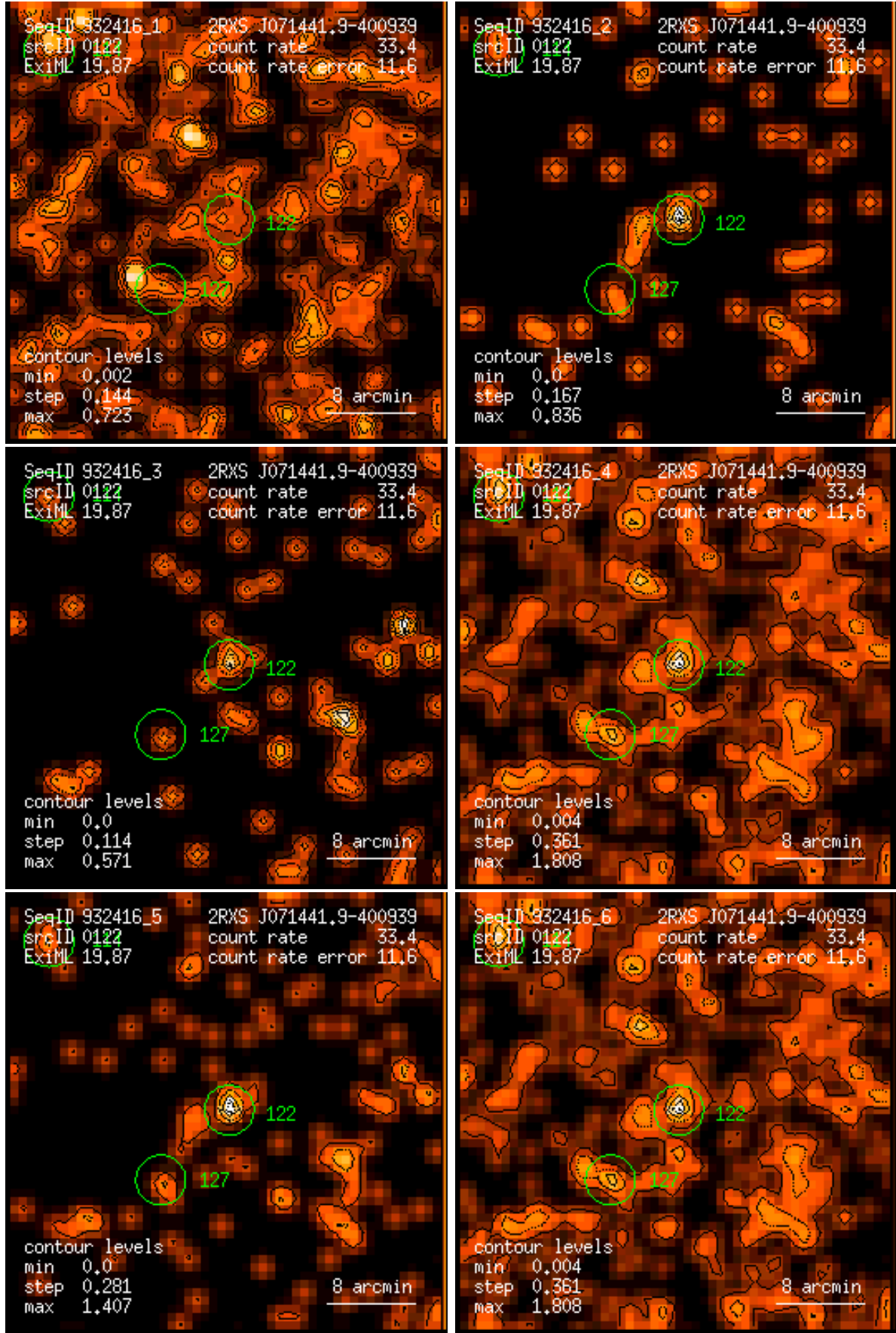
Figure 122: RASS 932416: detection 0122: band rate images, Gaussian filter: (1) PSPC channels 11 – 41, (2) 52 – 90, (3) 91 – 201, (4) 11 – 235, (5) 52 – 201, (6) 11 – 201. Broad band rates in counts/ks. Band rate contour levels in counts/ks/arcmin 2 .
