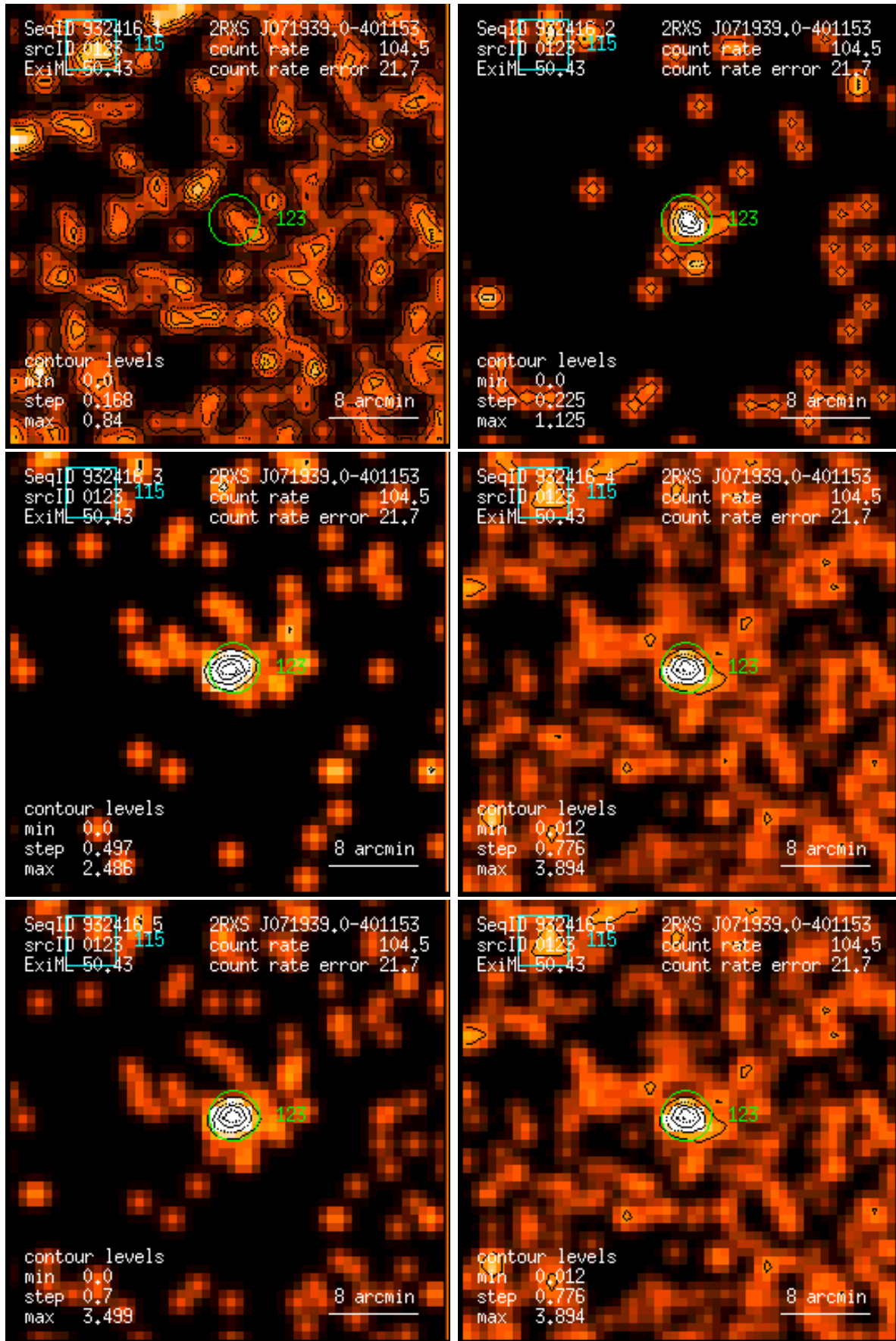
Figure 123: RASS 932416: detection 0123: band rate images, Gaussian filter: (1) PSPC channels 11 – 41, (2) 52 – 90, (3) 91 – 201, (4) 11 – 235, (5) 52 – 201, (6) 11 – 201. Broad band rates in counts/ks. Band rate contour levels in counts/ks/arcmin 2 .
