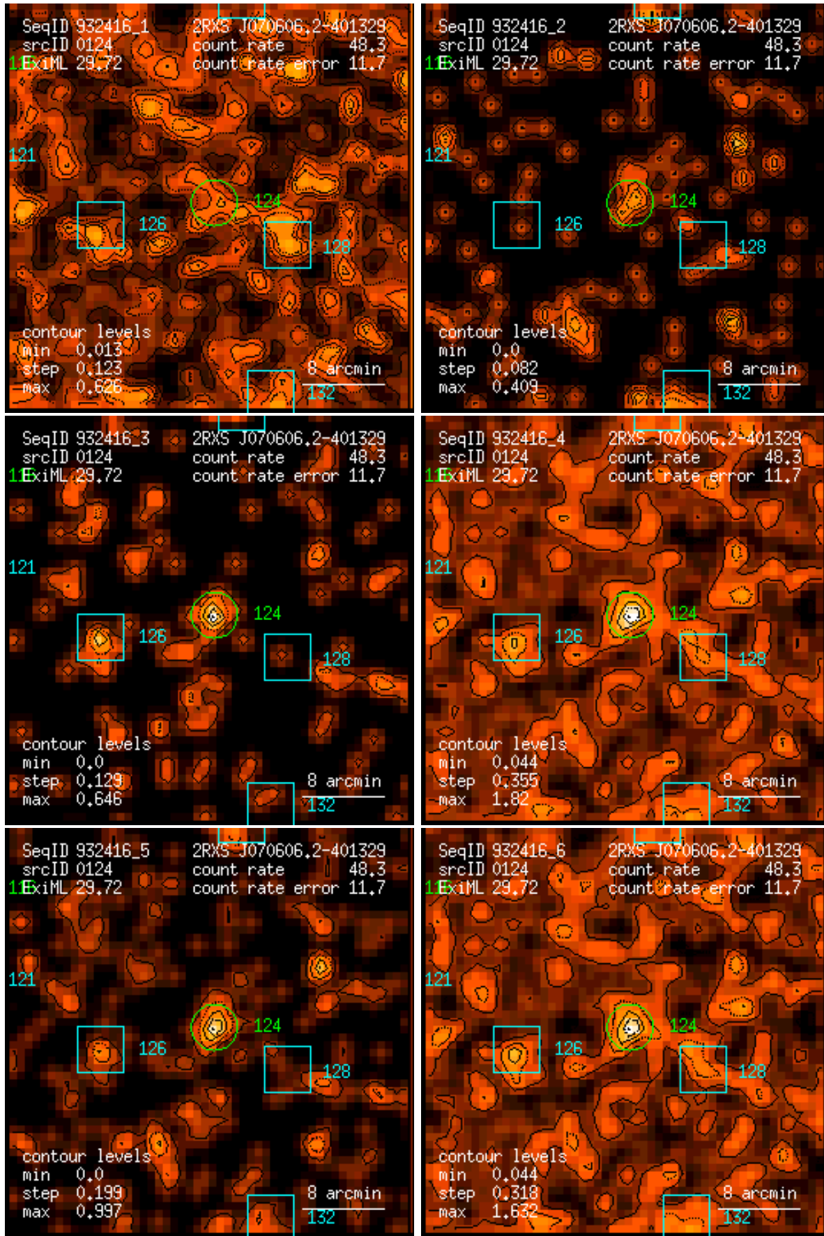
Figure 124: RASS 932416: detection 0124: band rate images, Gaussian filter: (1) PSPC channels 11 – 41, (2) 52 – 90, (3) 91 – 201, (4) 11 – 235, (5) 52 – 201, (6) 11 – 201. Broad band rates in counts/ks. Band rate contour levels in counts/ks/arcmin 2 .
