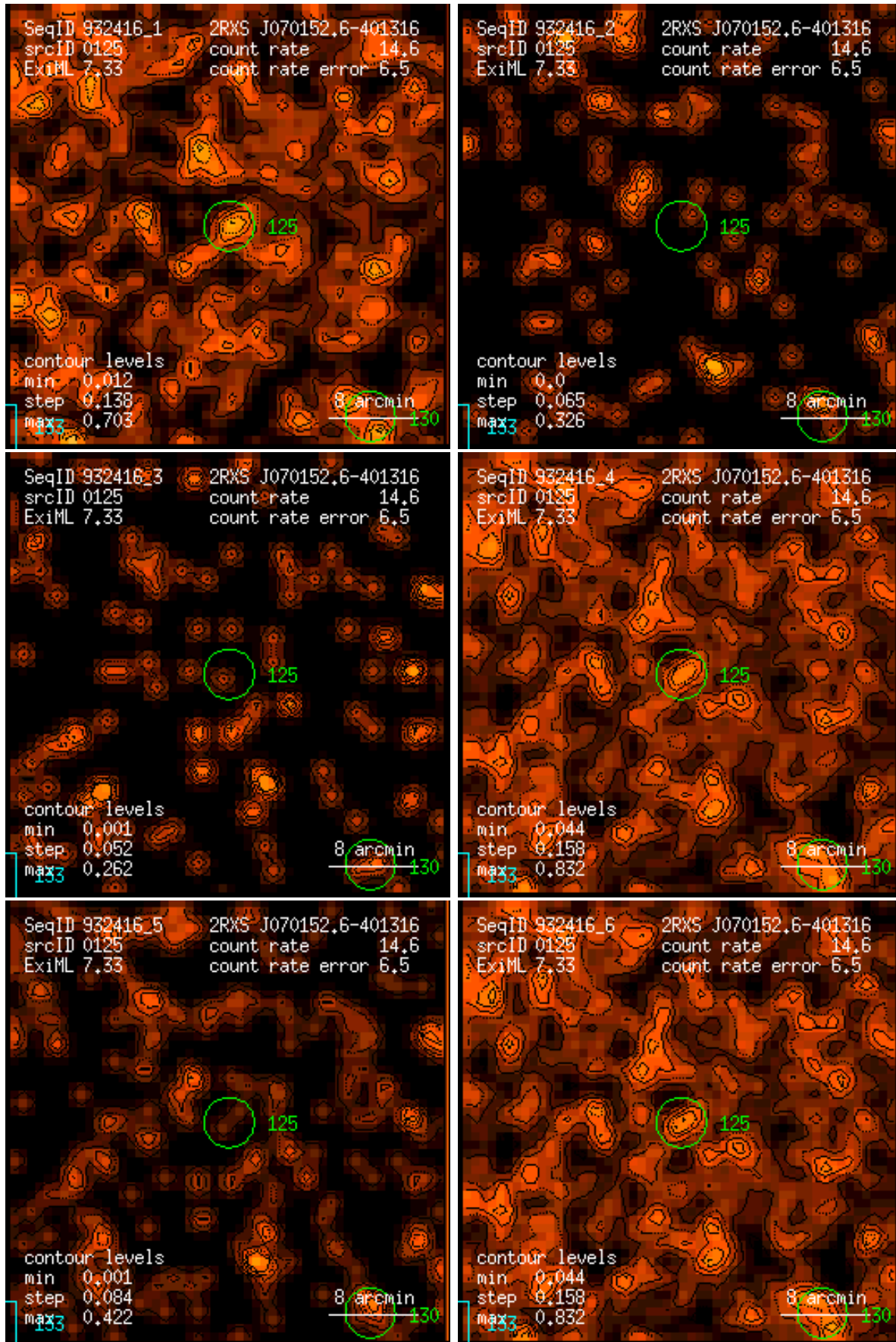
Figure 125: RASS 932416: detection 0125: band rate images, Gaussian filter: (1) PSPC channels 11 – 41, (2) 52 – 90, (3) 91 – 201, (4) 11 – 235, (5) 52 – 201, (6) 11 – 201. Broad band rates in counts/ks. Band rate contour levels in counts/ks/arcmin 2 .
