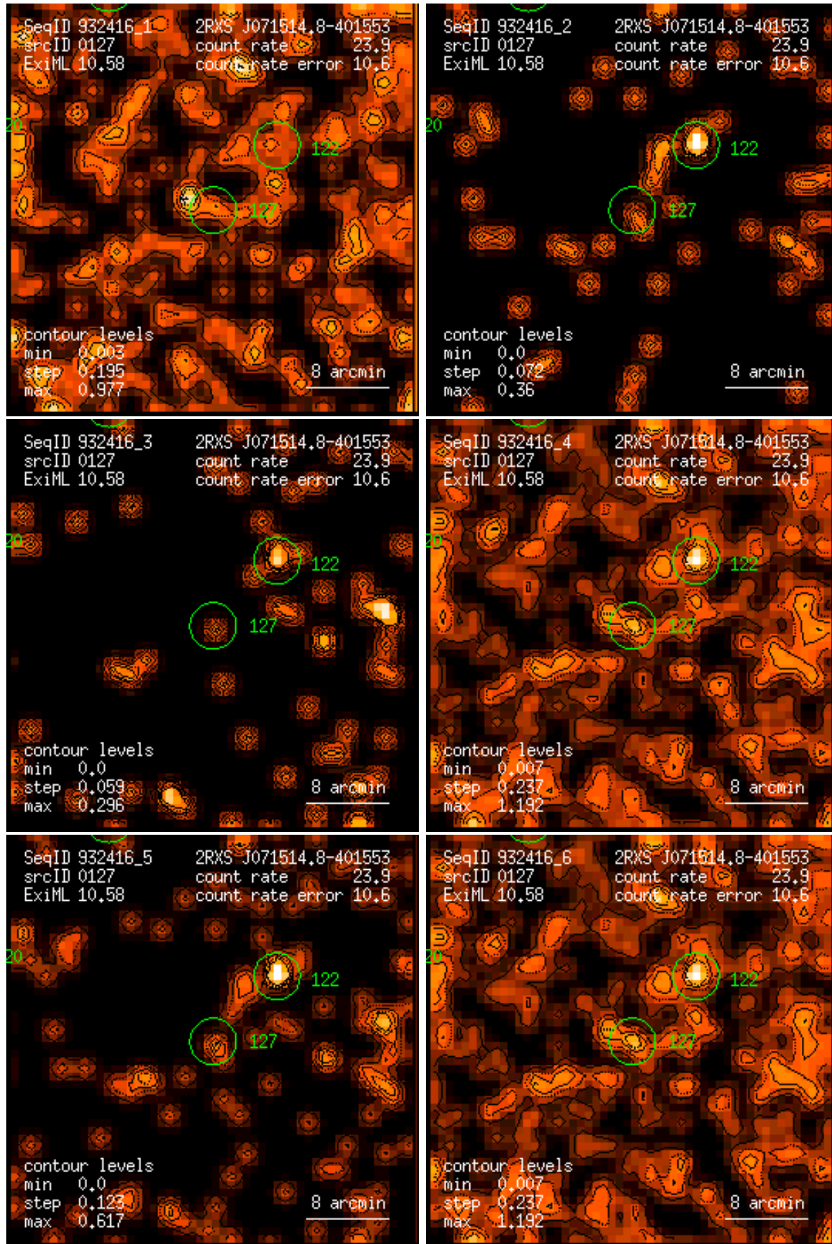
Figure 127: RASS 932416: detection 0127: band rate images, Gaussian filter: (1) PSPC channels 11 – 41, (2) 52 – 90, (3) 91 – 201, (4) 11 – 235, (5) 52 – 201, (6) 11 – 201. Broad band rates in counts/ks. Band rate contour levels in counts/ks/arcmin 2 .
