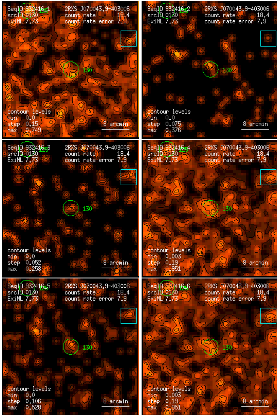
Figure 130: RASS 932416: detection 0130: band rate images, Gaussian filter: (1) PSPC channels 11 – 41, (2) 52 – 90, (3) 91 – 201, (4) 11 – 235, (5) 52 – 201, (6) 11 – 201. Broad band rates in counts/ks. Band rate contour levels in counts/ks/arcmin 2 .
